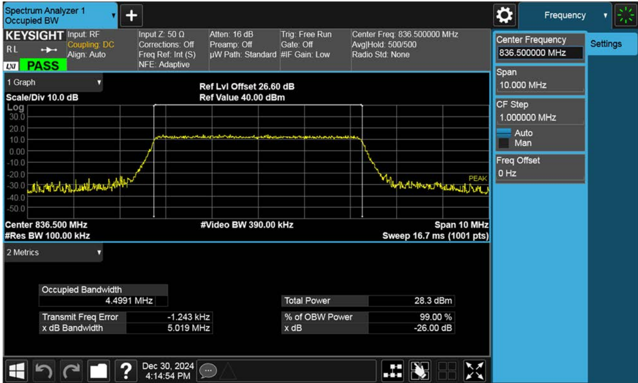
Occupied Bandwidth Plot (5 M BW Ch.167300 256QAM_RB 25_0)
