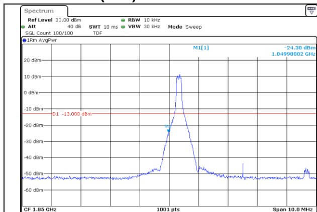
DFT-S-OFDM QPSK - Low Channel - 1 RB
