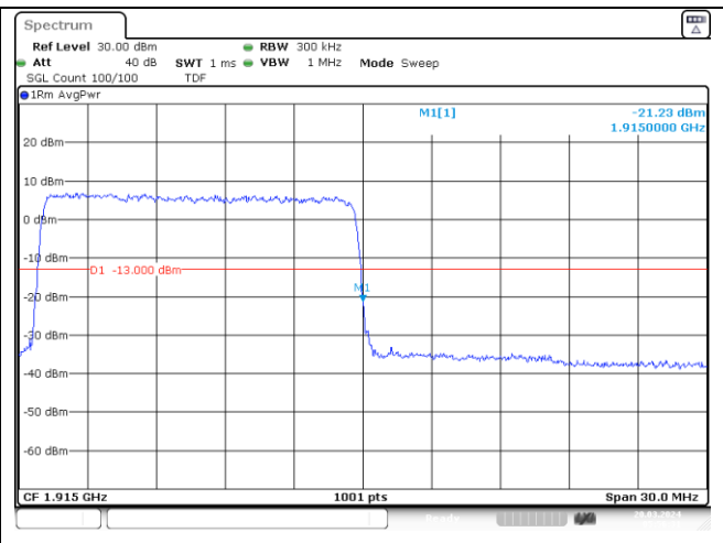
DFT-S-OFDM QPSK - High Channel - Full RB
