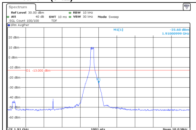
DFT-S-OFDM QPSK - High Channel - 1 RB
