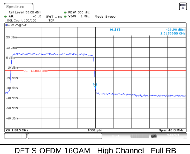
DFT-S-OFDM 16QAM - High Channel - Full RB
