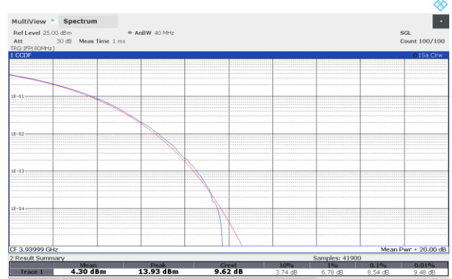
40 MHz Middle Channel - CP-OFDM 256QAM
