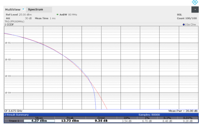
50 MHz Middle Channel - CP-OFDM 256QAM
