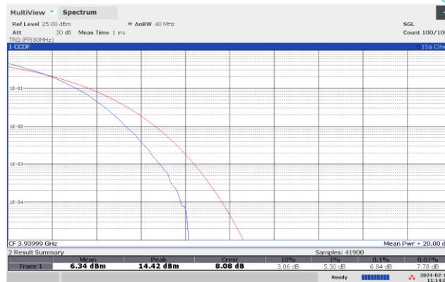
40 MHz Middle Channel - DFT-S-OFDM 256QAM
