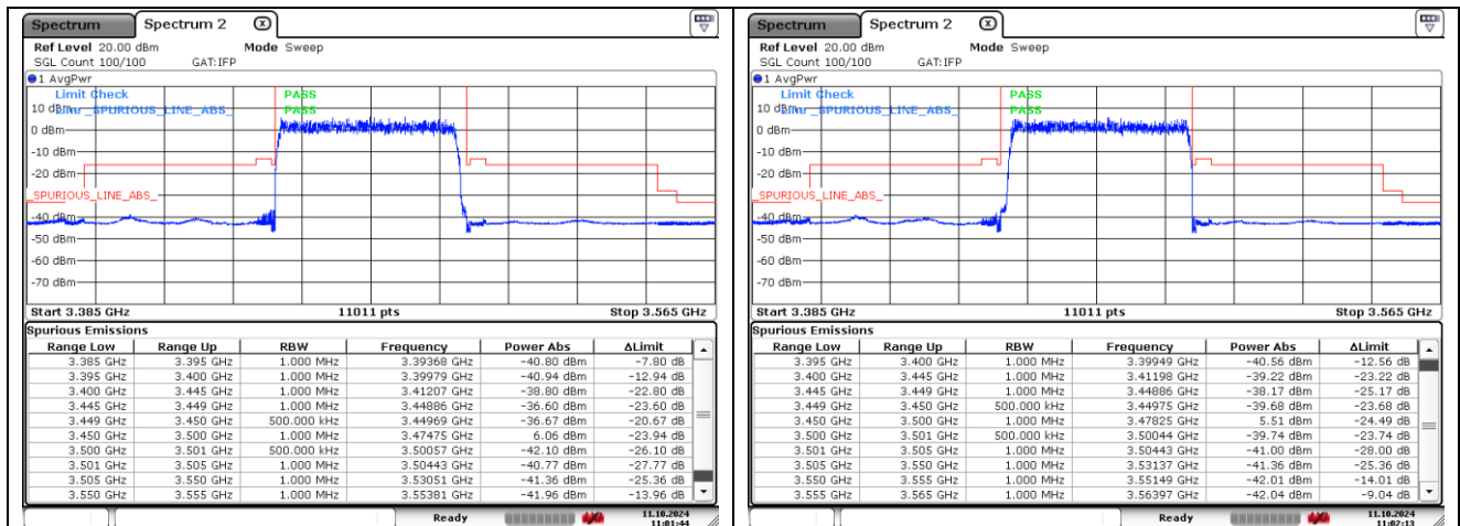
DFT-S-OFDM 16QAM Low Channel - Full RB
