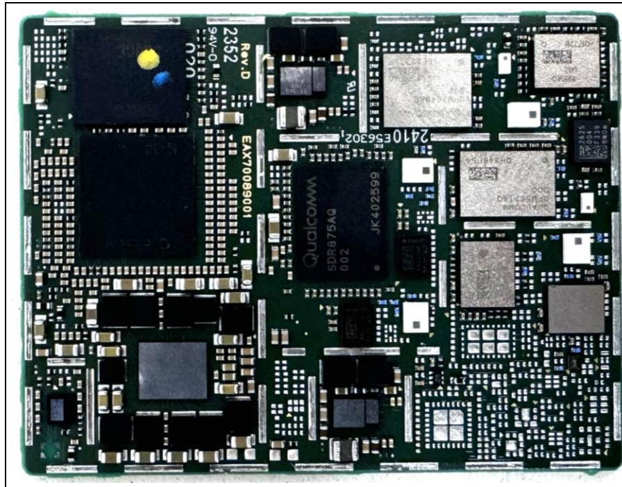
Bottom view of Main PCB
