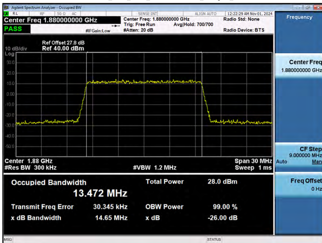
LTE2_15 M_OBW_Middle Channel_256QAM_FullRB
