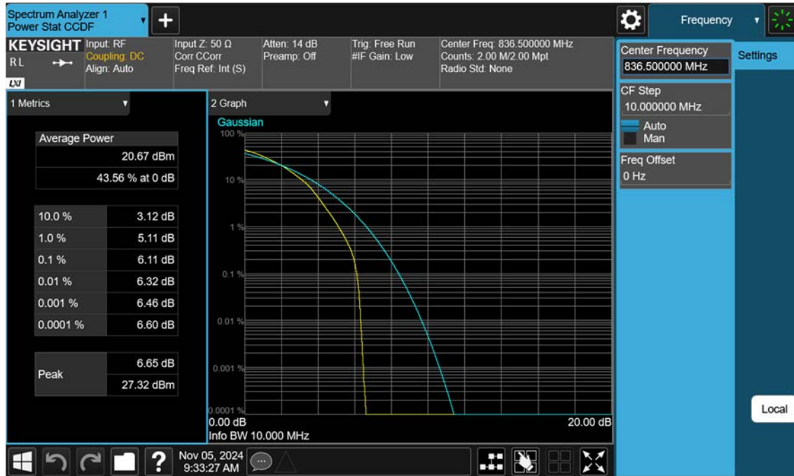
NR5_10 M_PAR_Mid_64QAM_FullRB
