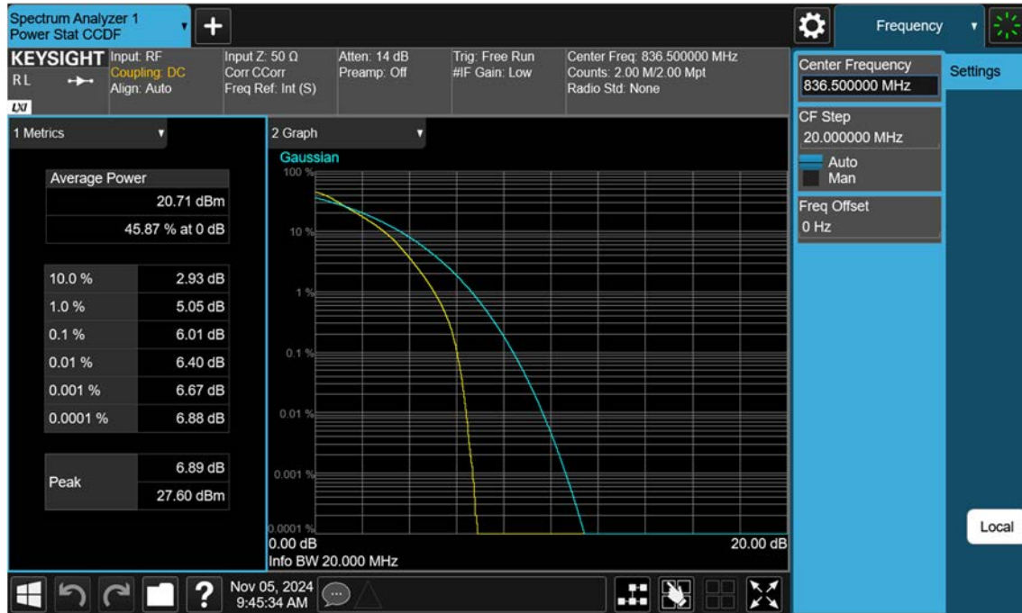
NR5_20 M_PAR_Mid_64QAM_FullRB
