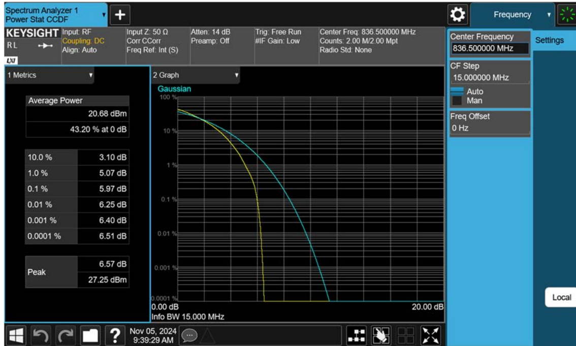
NR5_15 M_PAR_Mid_64QAM_FullRB
