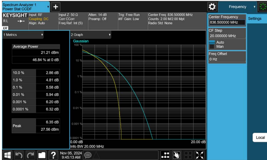
NR5_20 M_PAR_Mid_16QAM_FullRB
