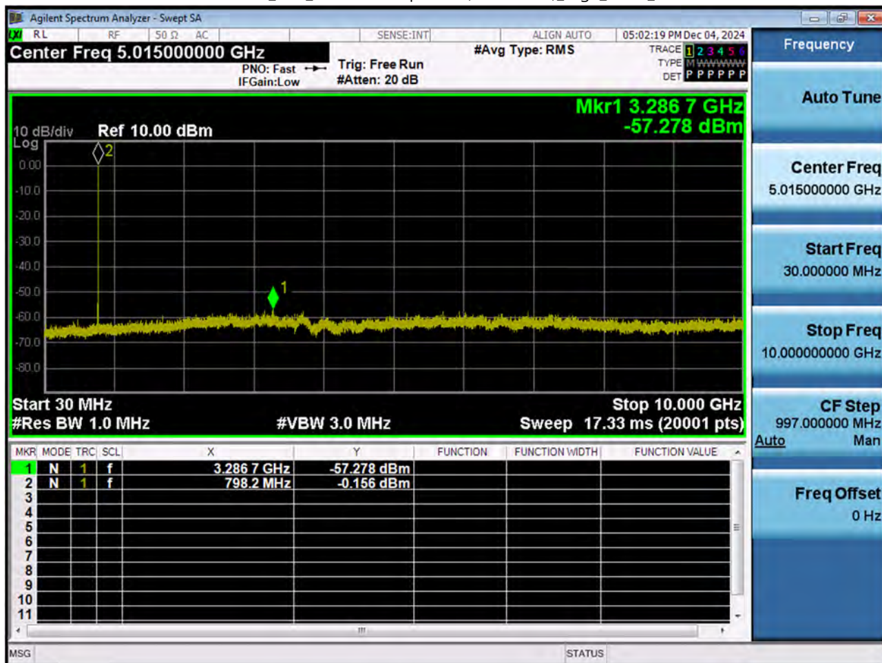
LTE B14_5 M_Conducted Spurious(30 M-10 G)_High_QPSK_1RB
