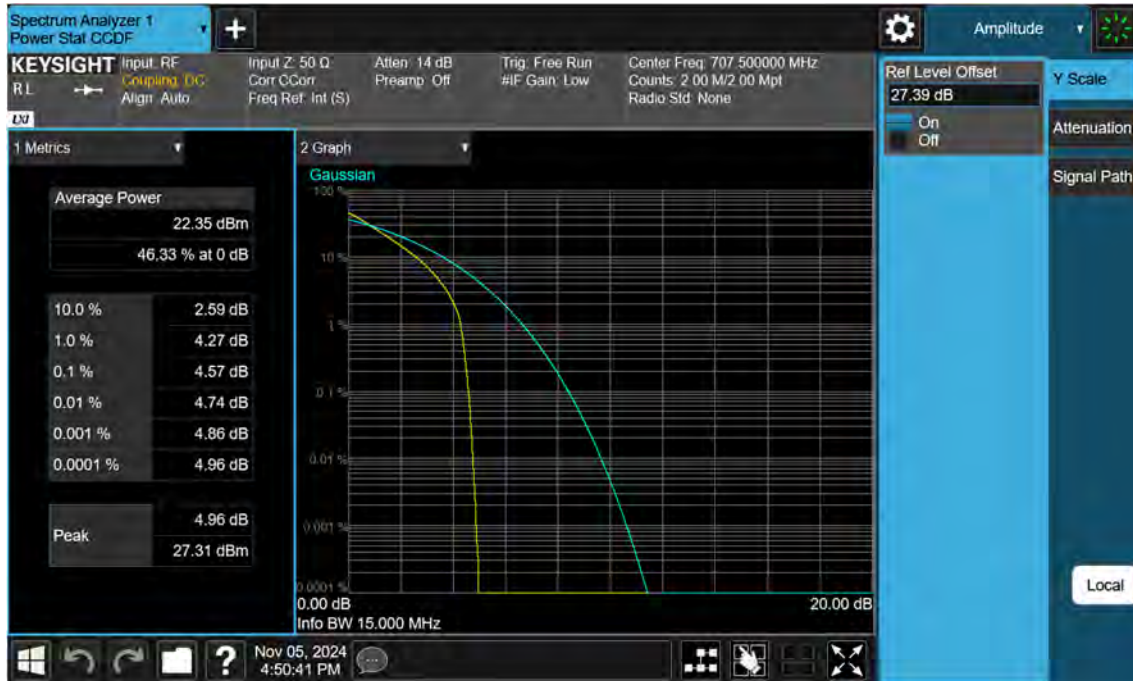
NR12_15 M_PAR_Mid_QPSK_FullRB
