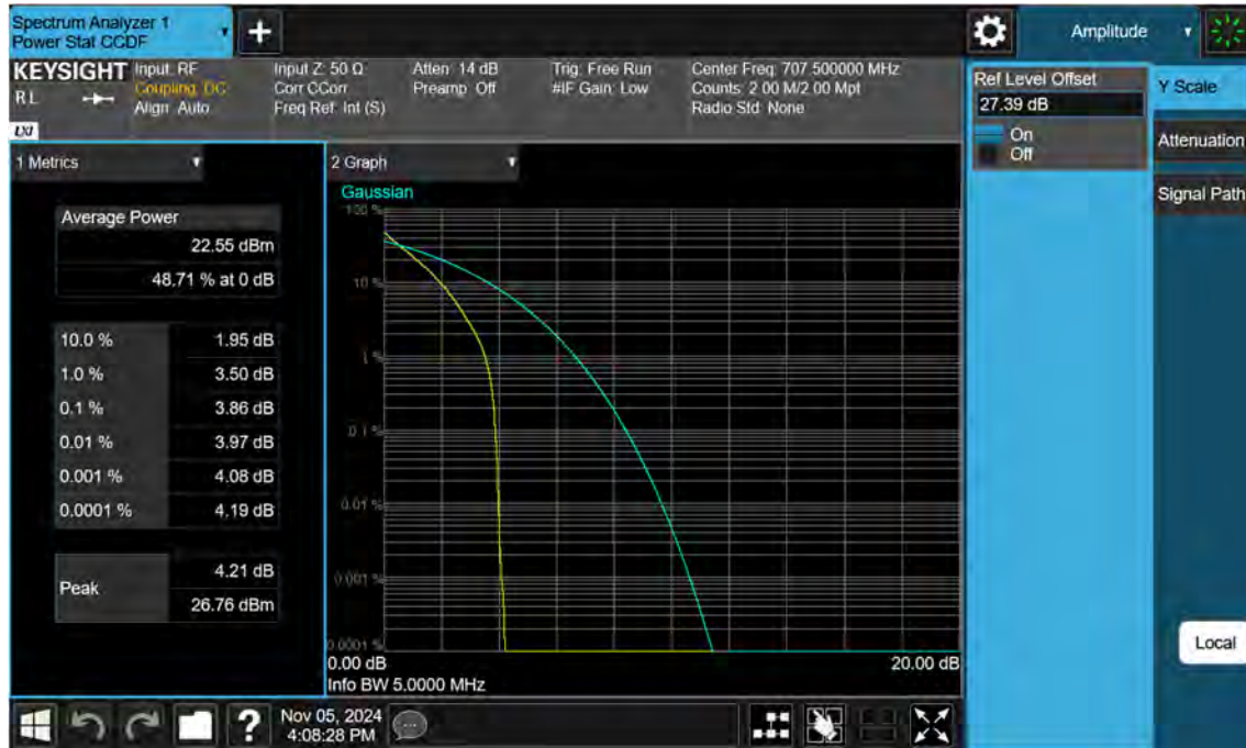
NR12_5 M_PAR_Mid_BPSK_FullIRB
