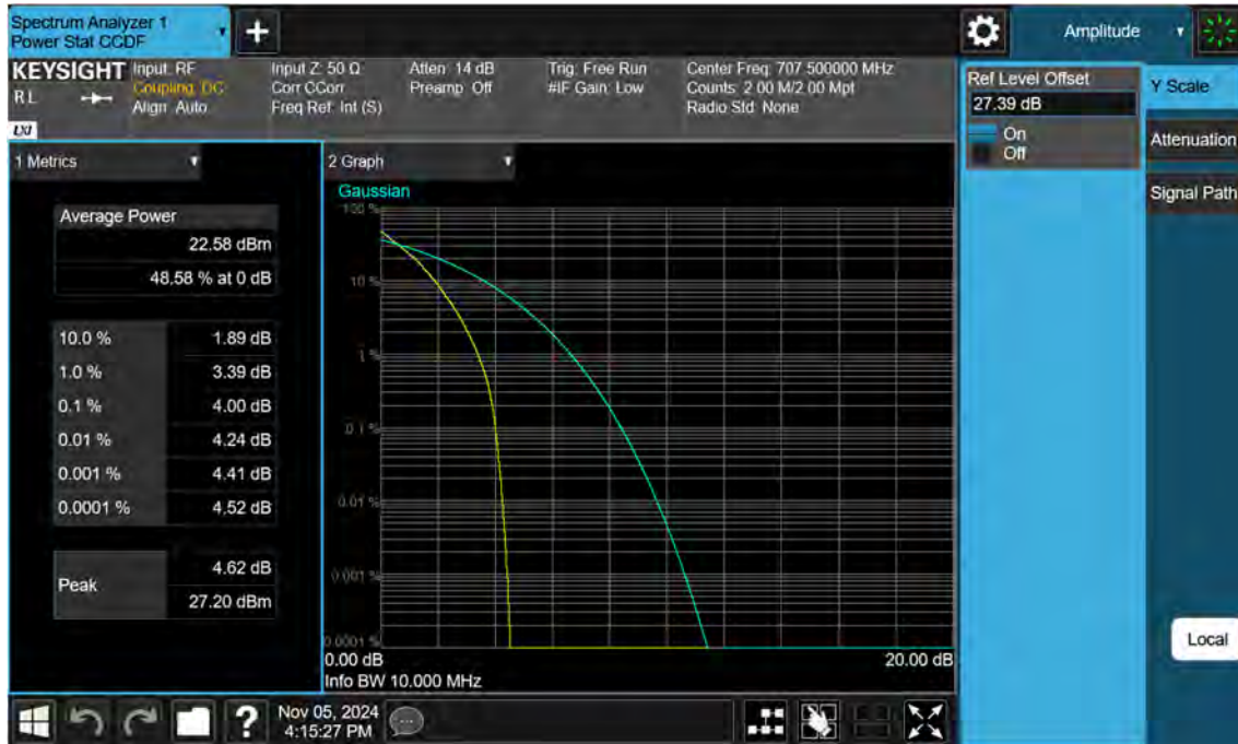
NR12_10 M_PAR_Mid_BPSK_FullIRB
