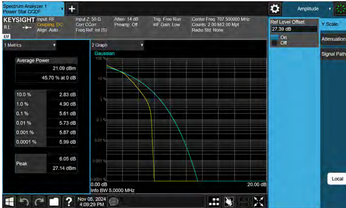
NR12_5 M_PAR_Mid_16QAM_FullRB
