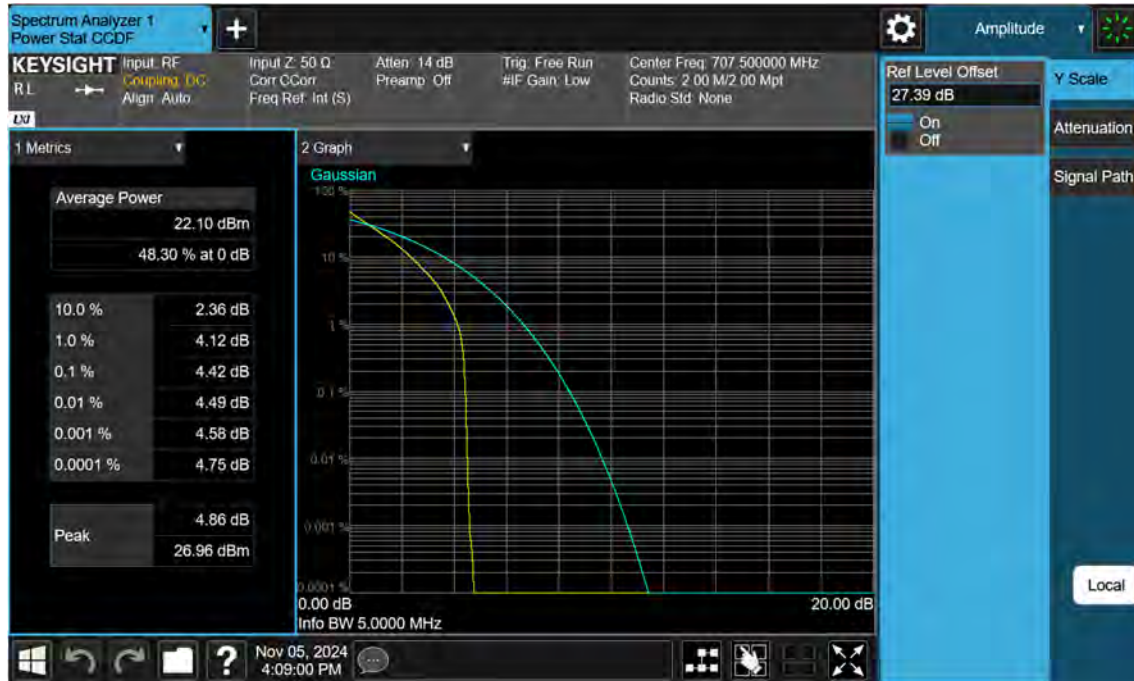
NR12_5 M_PAR_Mid_QPSK_FullRB
