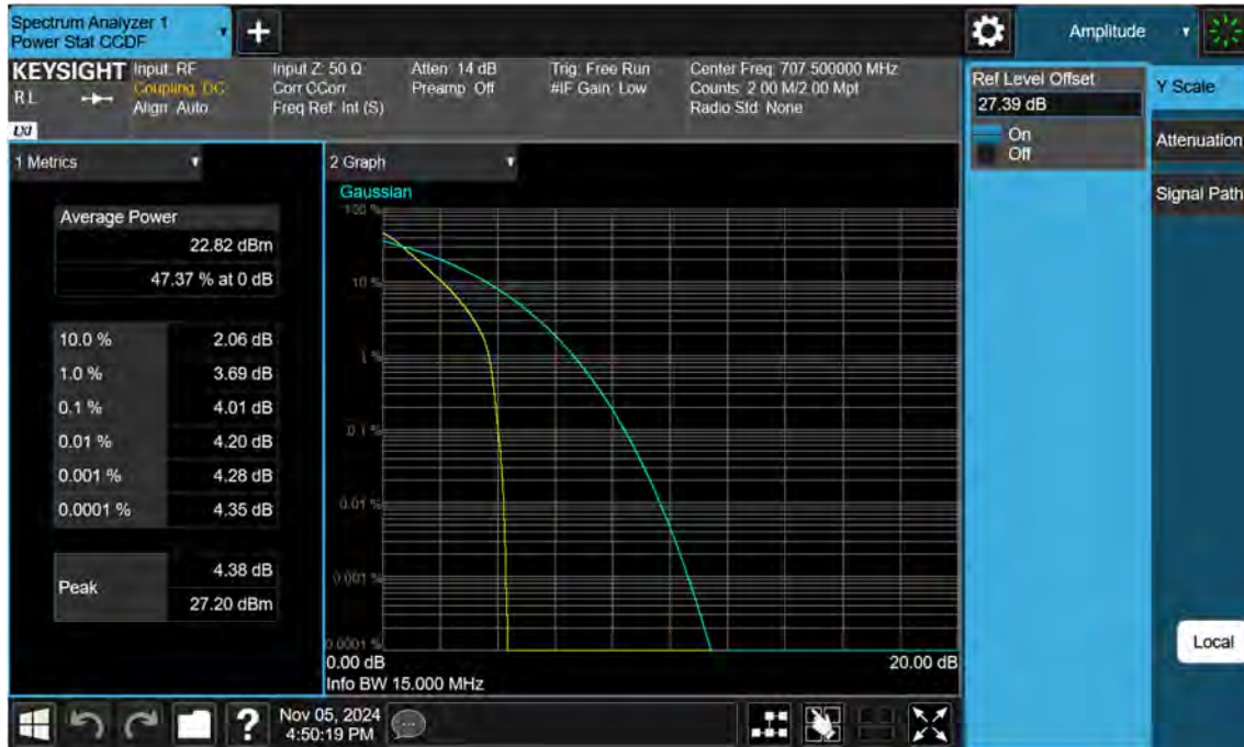
NR12_15 M_PAR_Mid_BPSK_FullIRB
