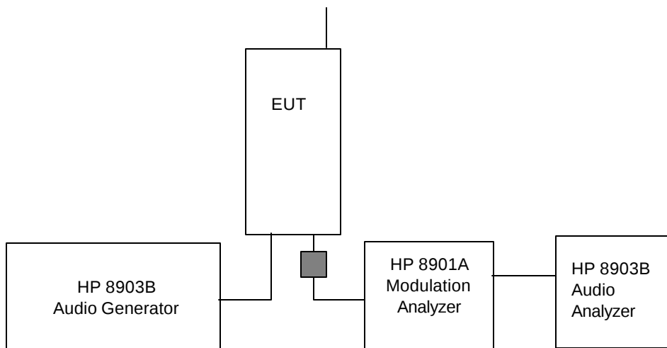
Fig. 3. Transmitter Audio Frequency & Tone Modulation Test Setup.
