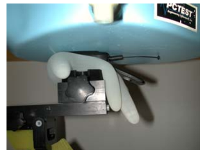
Figure 24. Hand SAR Test Setup
