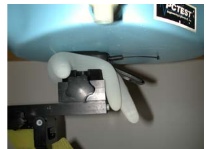
Figure 25. Hand SAR Test Setup
