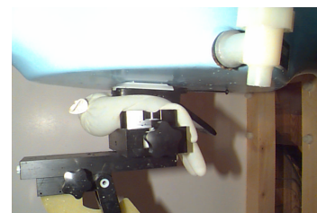
Figure 23. Hand SAR Test Setup
