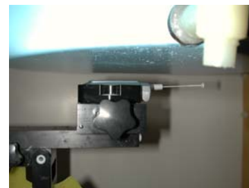
Figure 21. Body SAR Test Setup without Holster
