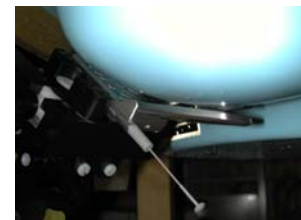
Figure 19. Head SAR Test Setup
