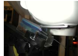
Figure 14.6 Left Head SAR Test Setup -- Cheek / Touch Position --
