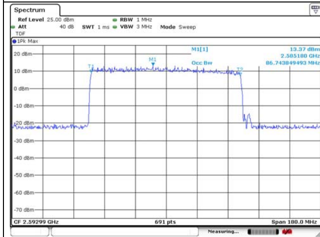
90 MHz DFT-S-OFDM 16QAM Middle Channel – Full RB
