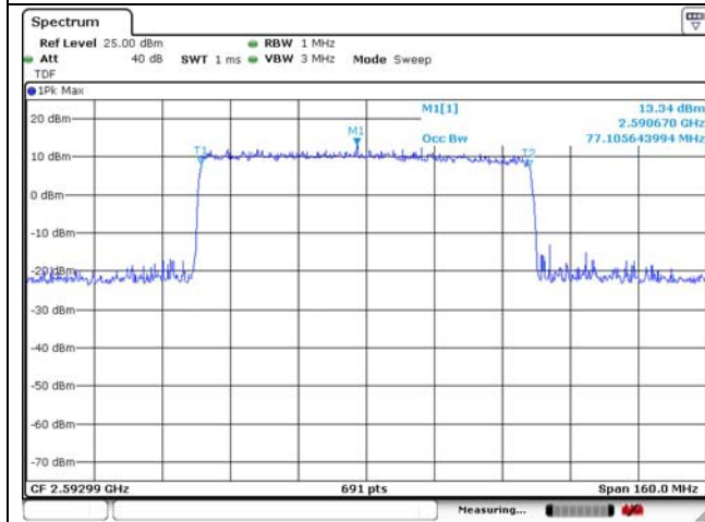
80 MHz DFT-S-OFDM 16QAM Middle Channel – Full RB
