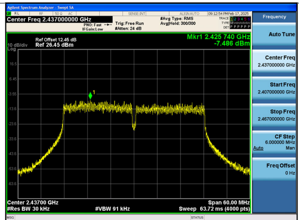
802.11n_HT40-CH 6
