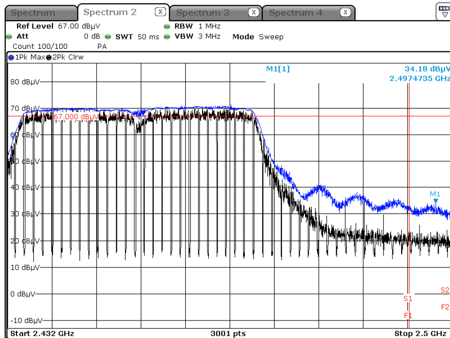
Radiated Restricted Band Edges plot – Peak Result (802.11n (HT40)_MCS0, Ch.9, Y-H)
