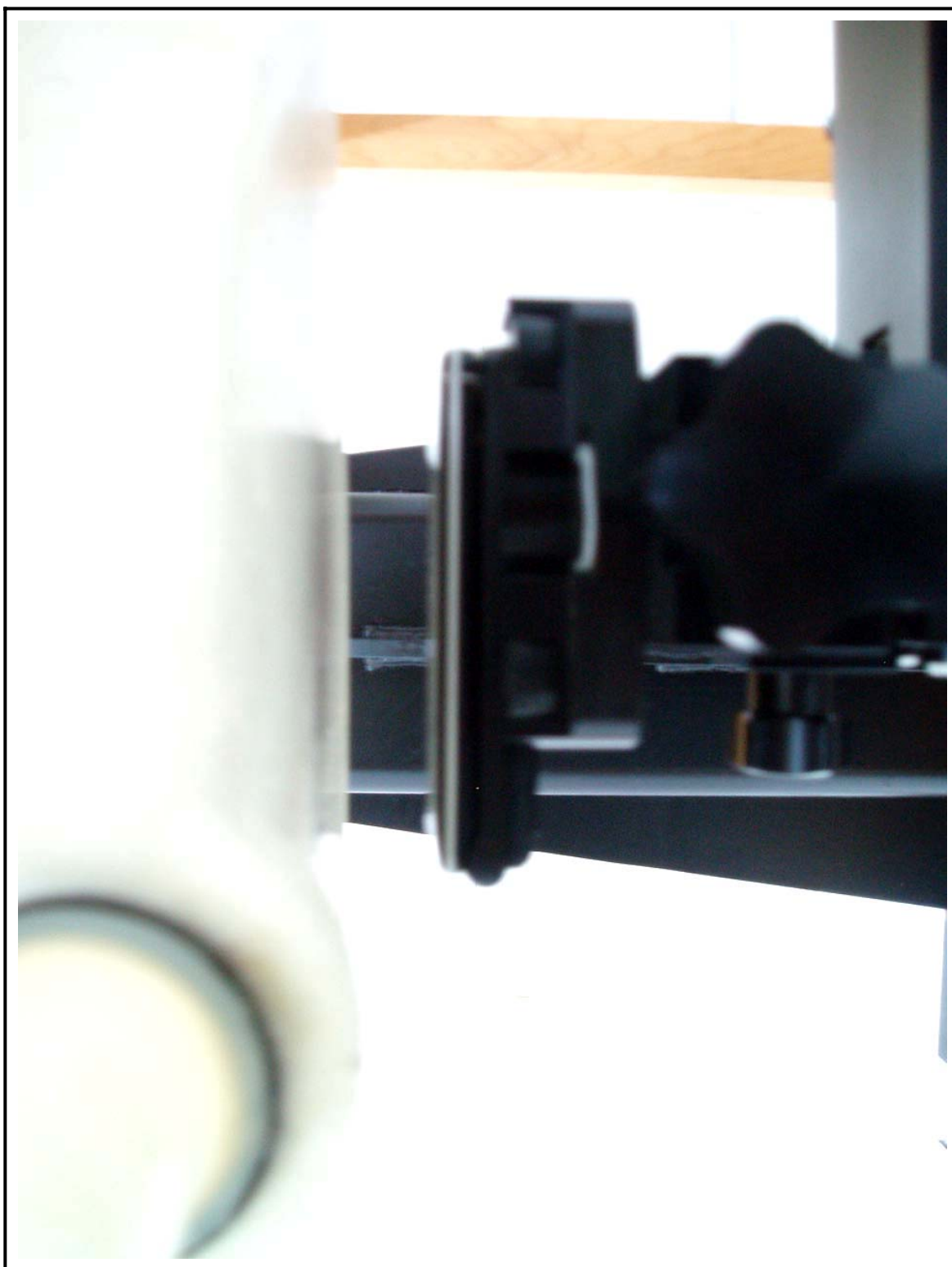
Figure 12 Body SAR Test Setup – w/o Holster
