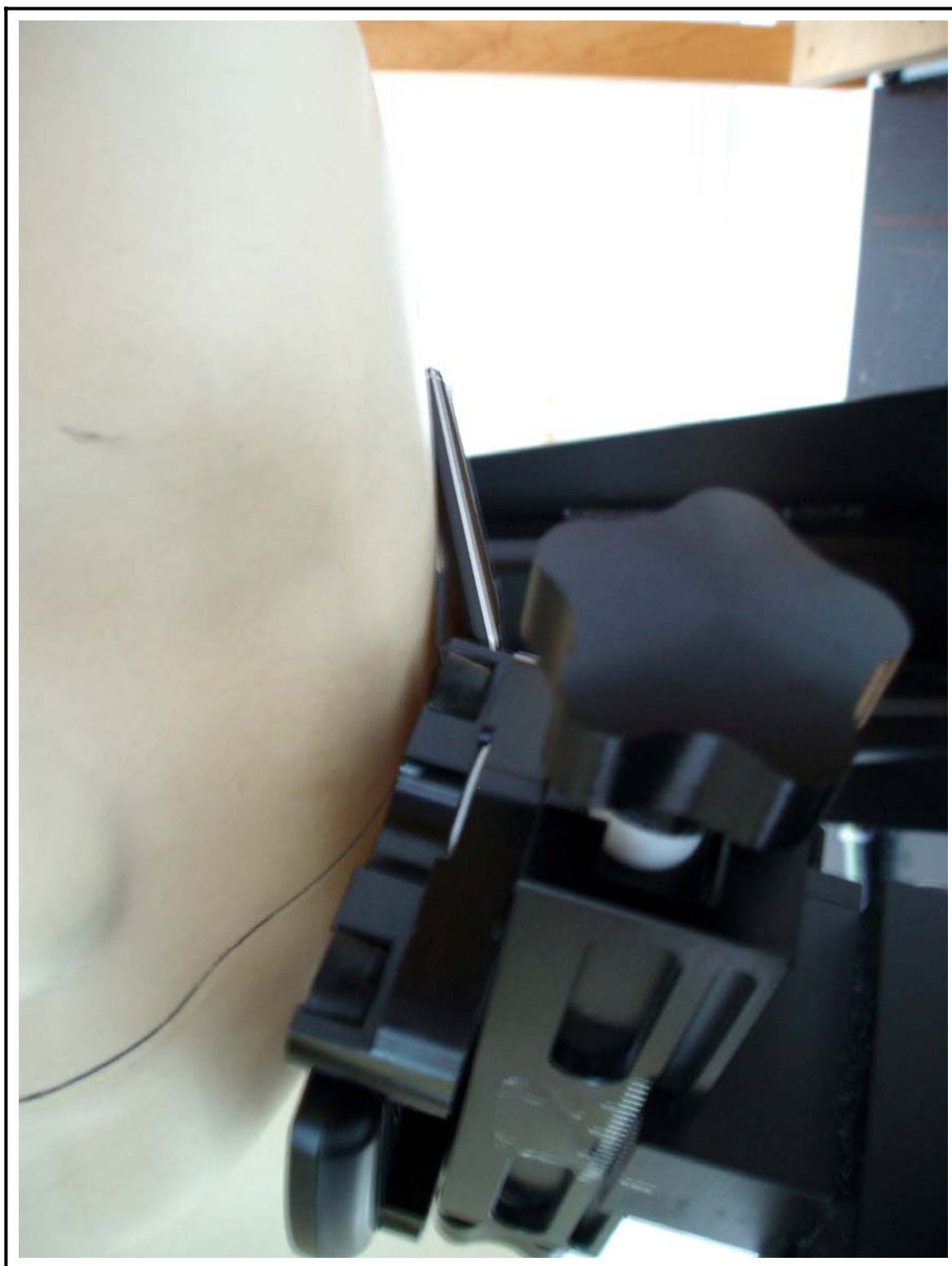
Figure 5 Left Head SAR Test Setup – Ear Touch Position
