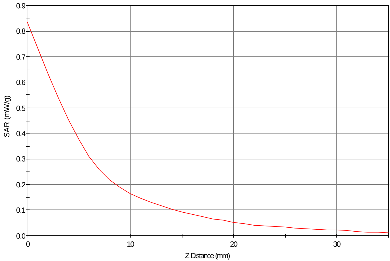
SAR - Z Axis at Hotspot x:-7.0 y:25.0
