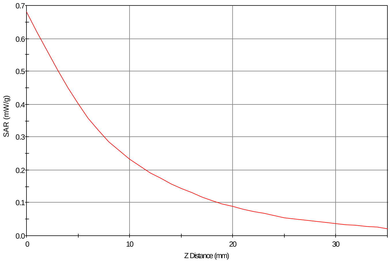
SAR - Z Axis at Hotspot x:68.0 y:-1.0
