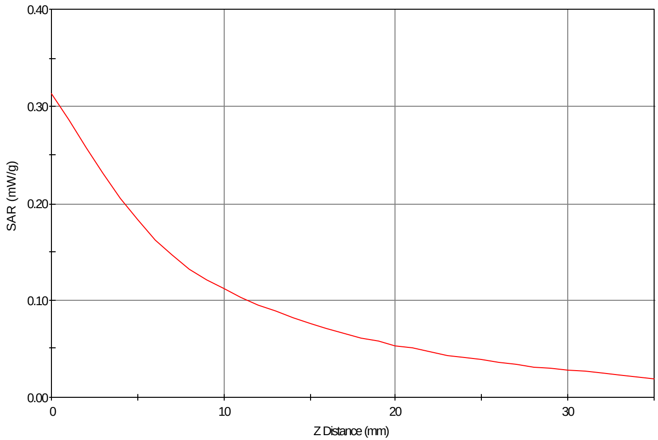
SAR - Z Axis at Hotspot x:-2.0 y:-13.0
