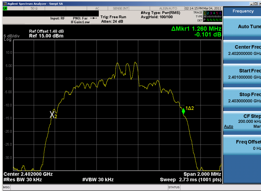
Plot 6-7. 20dB Bandwidth Plot (Bluetooth, 3Mbps – Ch. 0)
