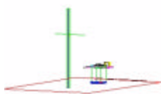
Figure 3-1. 3-Meter Test Site
