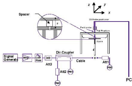
Figure 12-1 System Verification Setup Diagram
