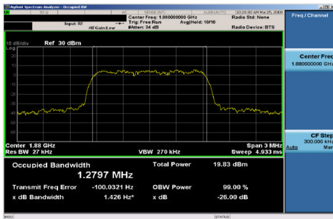
Plot 7-18. Occupied Bandwidth Plot (PCS CDMA Mode – Ch. 600)
