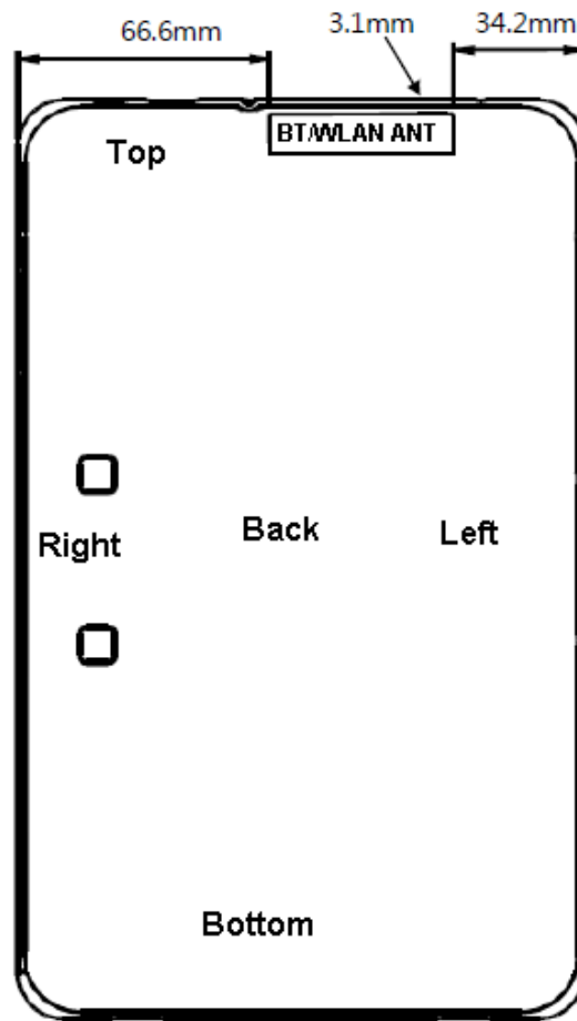
Figure 10-1 Antenna & Key feature Diagram
