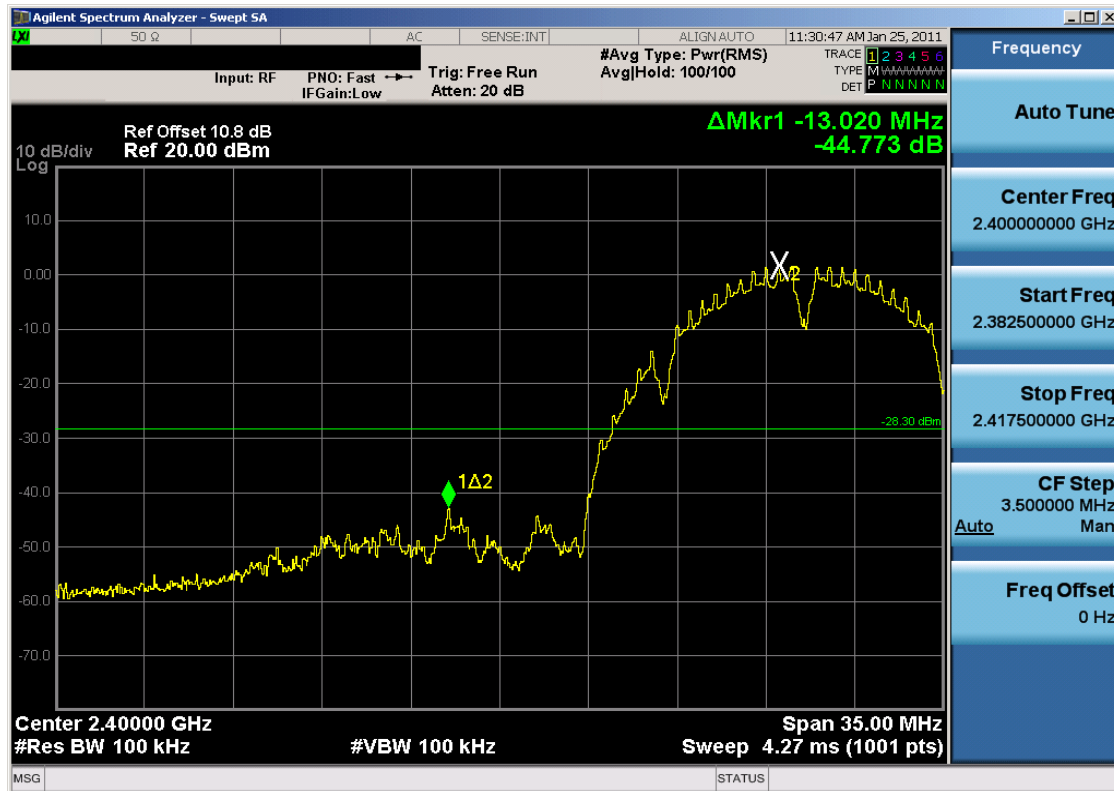
Plot 6-19. Band Edge Plot (802.11b – Ch. 1)
