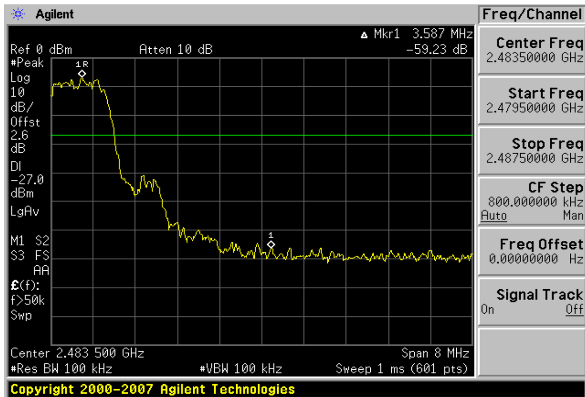
Plot 6-13. Band Edge Plot (Bluetooth, 2Mbps – Ch. 78)
