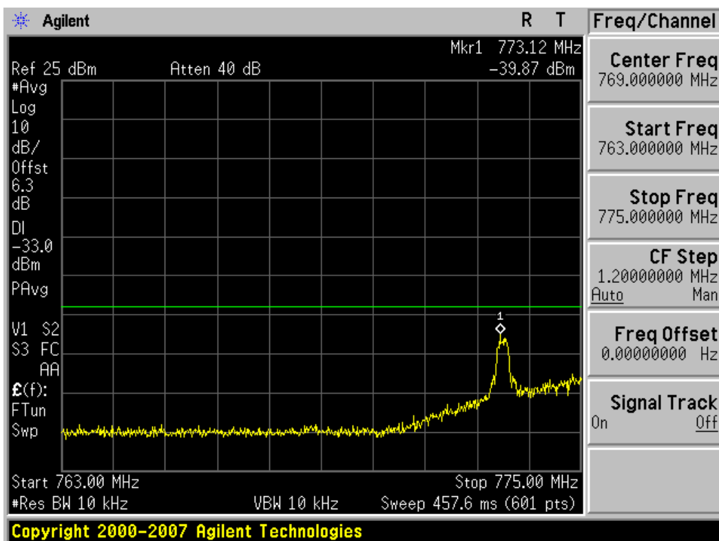
Plot 7-3 Lower Emission Mask (763 – 775MHz) Plot (QPSK – RB Size 1, RB Offset 0)
