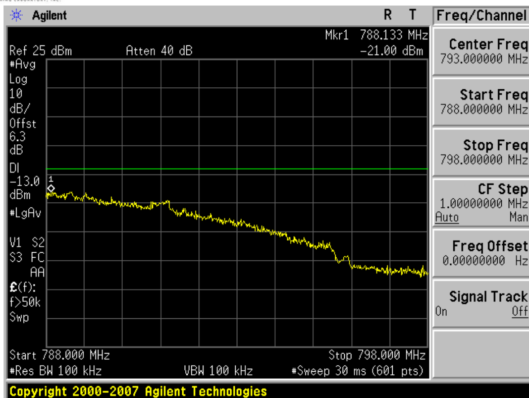
Plot 7-6 Upper Band Edge Plot (QPSK - RB Size 50, RB Offset 0)
