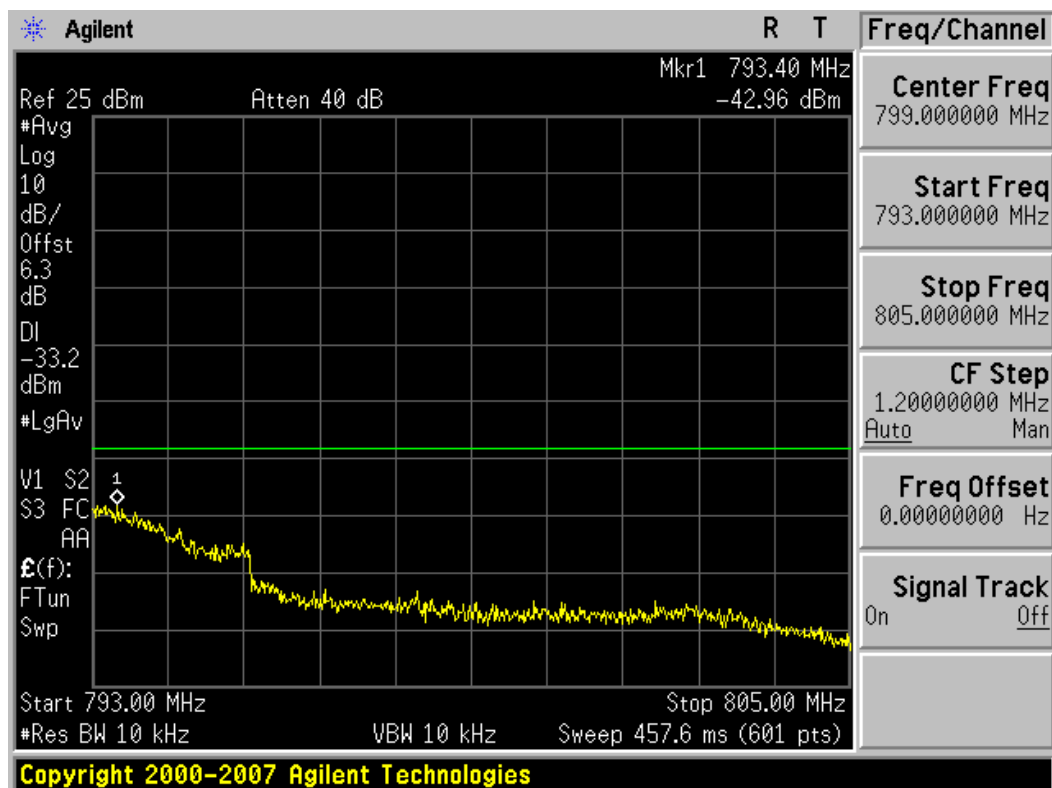
Plot 7-8 Upper Emission Mask (793 – 805MHz) Plot (QPSK – RB Size 50, RB Offset 0)
