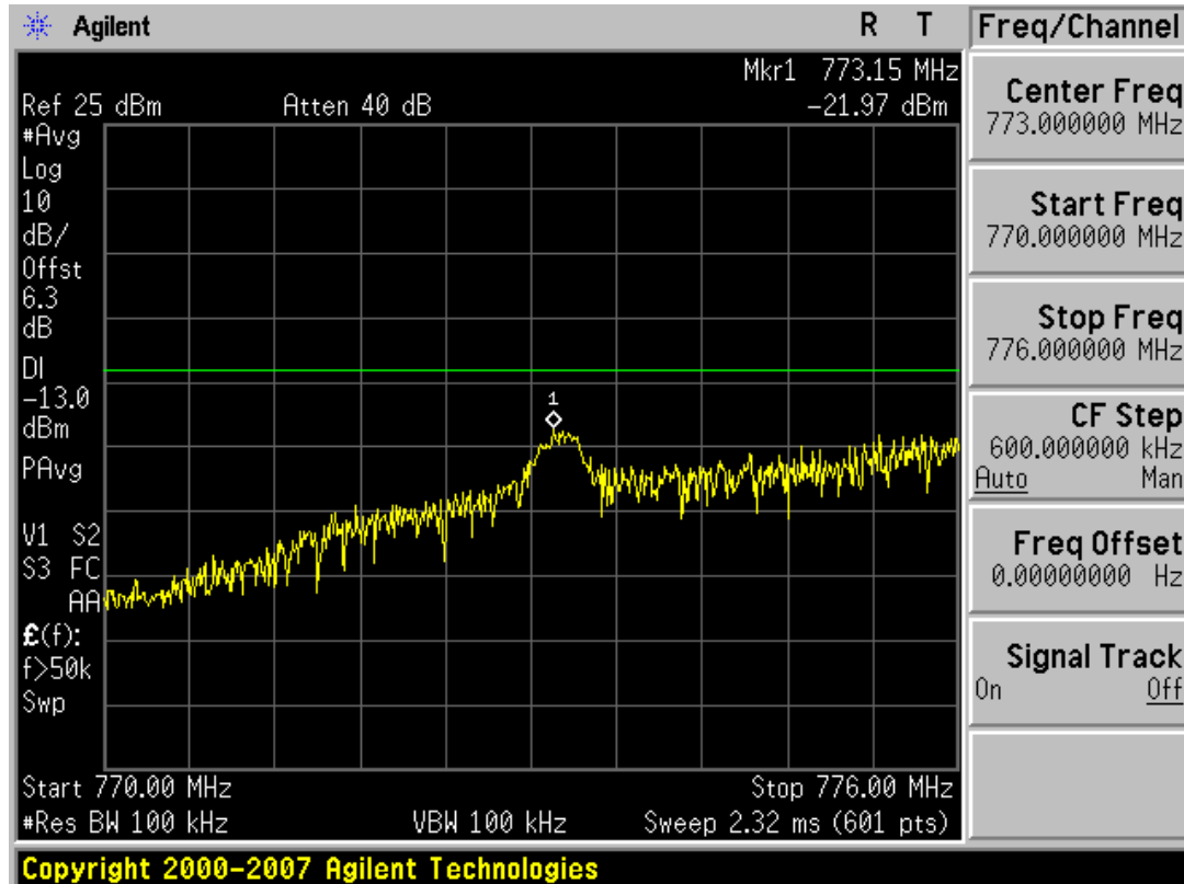
Plot 7-1 Lower Band Edge (QPSK – RB Size 1, RB Offset 0)
