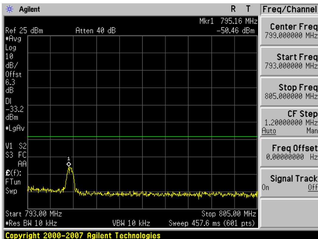
Plot 7-7 Upper Emission Mask (793 - 805MHz) Plot (QPSK - RB Size 1, RB Offset 0)
