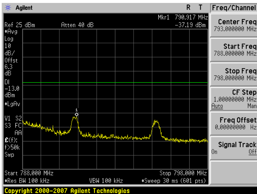
Plot 7-5 Upper Band Edge Plot (QPSK - RB Size 1, RB Offset = 49)
