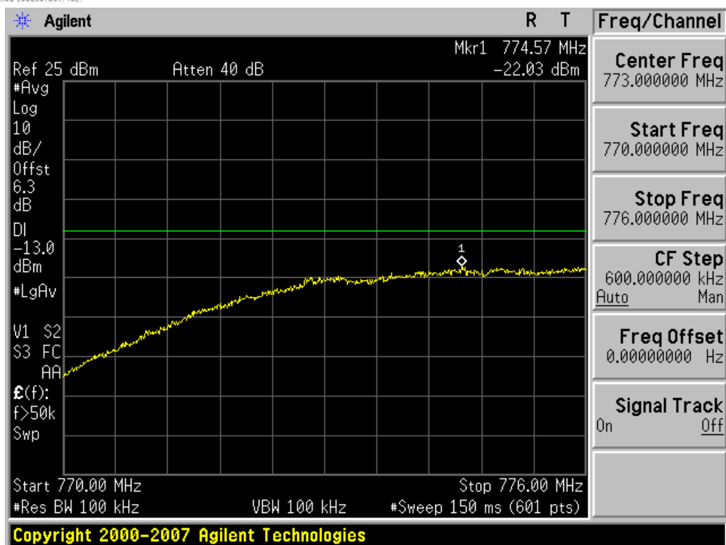
Plot 7-2 Lower Band Edge (QPSK – RB Size 50, RB Offset 0)
