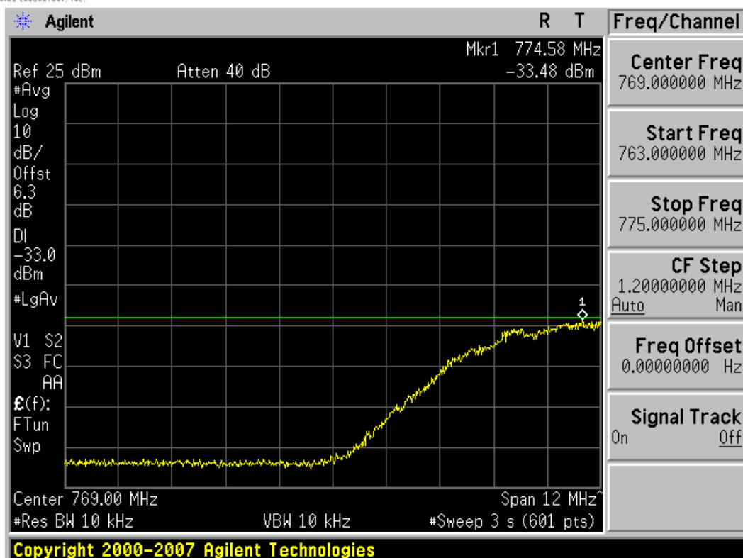
Plot 7-4 Lower Emission Mask (763 - 775MHz) Plot (QPSK - RB Size 50, RB Offset 0)
