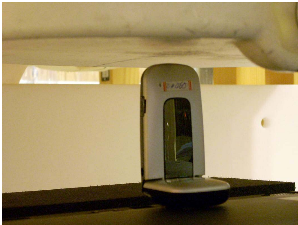
Figure 18-5 SAR Test Setup Photo 5
