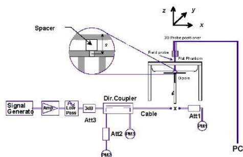
Figure 12-1 System Verification Setup Diagram
