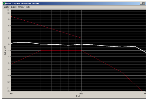
Figure 6-1 Axial Frequency Response
