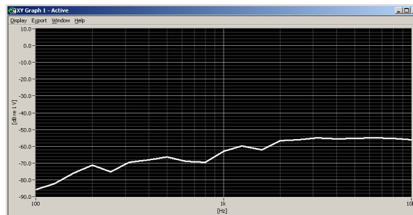
Figure 6-2 Worst-case ABM2 Plot for WD
