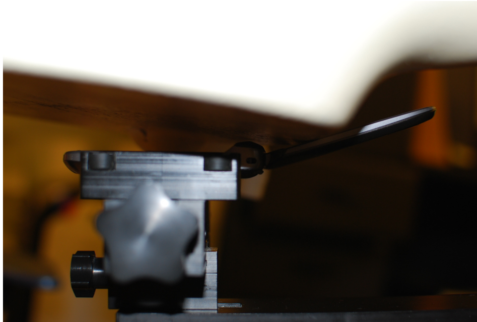
SAR Test Setup Photo 1 – Mouth Jaw at 2.54 cm
