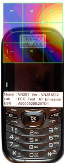
Figure 17-4 E-Field WD Scan overlay
