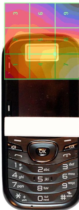
Figure 17-5 H-Field WD Scan overlay
