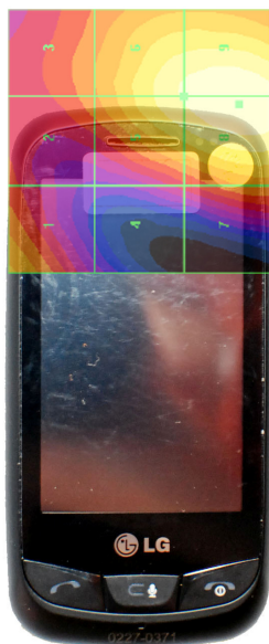
Figure 17-4 E-Field WD Scan overlay
