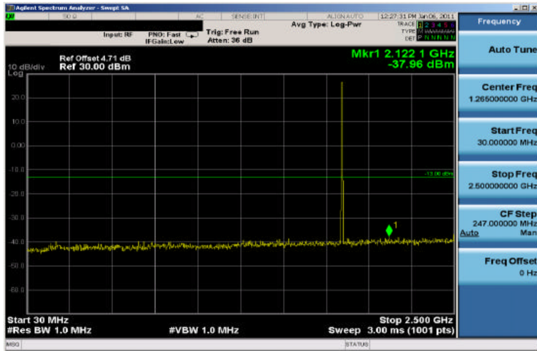
Plot 7-1. Conducted Spurious Plot (PCS CDMA Mode – Ch. 25)
