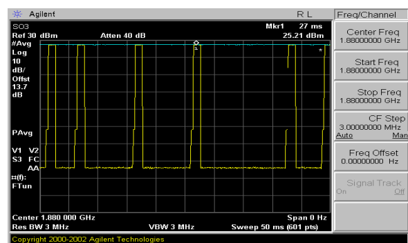
Figure 8-4 Zero-Span Plots
