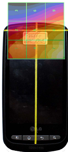
Figure 17-5 H-Field WD Scan overlay
