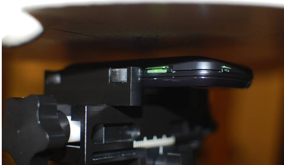
SAR Test Setup Photo 5 – Body Back at 1.0 cm
