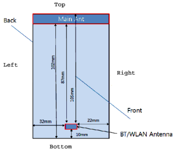
Figure 11-1 Identification of Sides for SAR Testing
