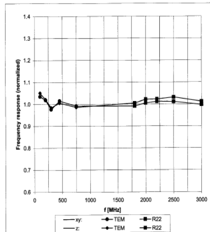
Figure 5-4 H-Field Probe Frequency Response
