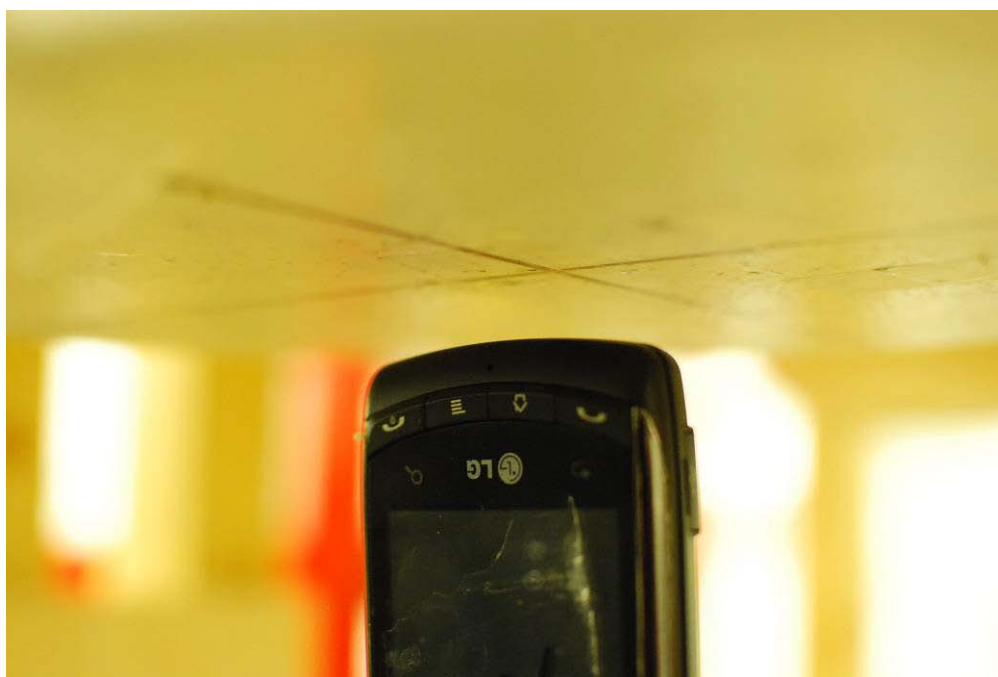
Figure 19-4 SAR Test Setup Photo 4 – Bottom at 1.0 cm
