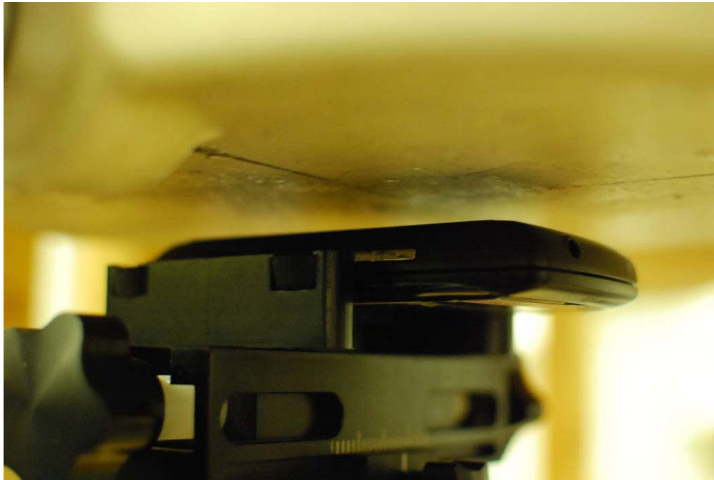
Figure 19-1 SAR Test Setup Photo 1 – Back at 1.0 cm
