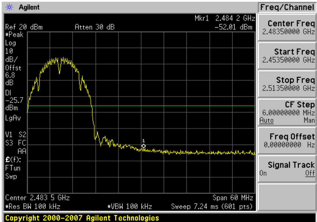
Plot 6-8. Band Edge Plot (802.11b – Ch. 11)
