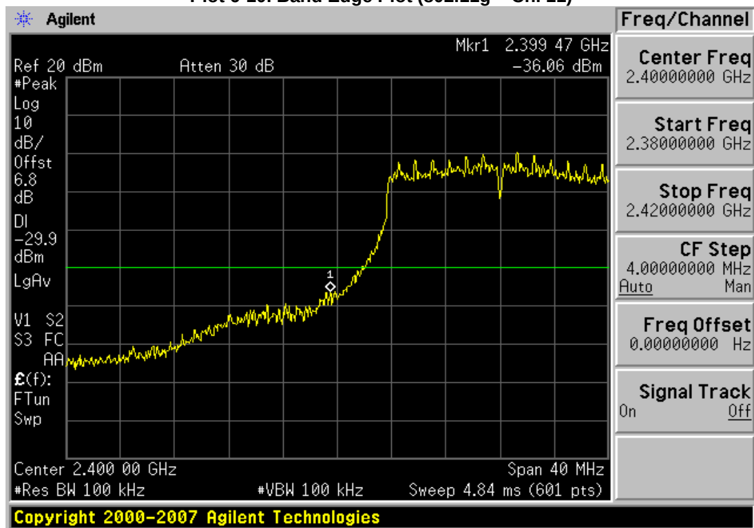
Plot 6-11. Band Edge Plot (802.11n – Ch. 1)
