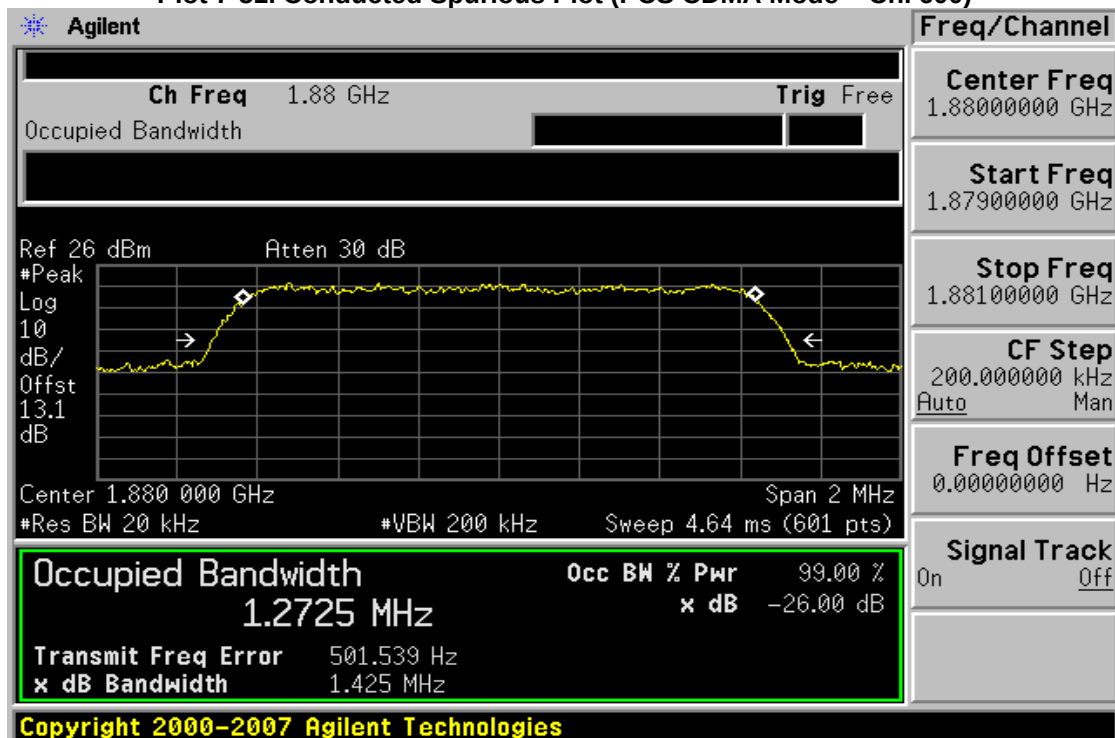
Plot 7-52. Occupied Bandwidth Plot (PCS CDMA Mode – Ch. 600)
