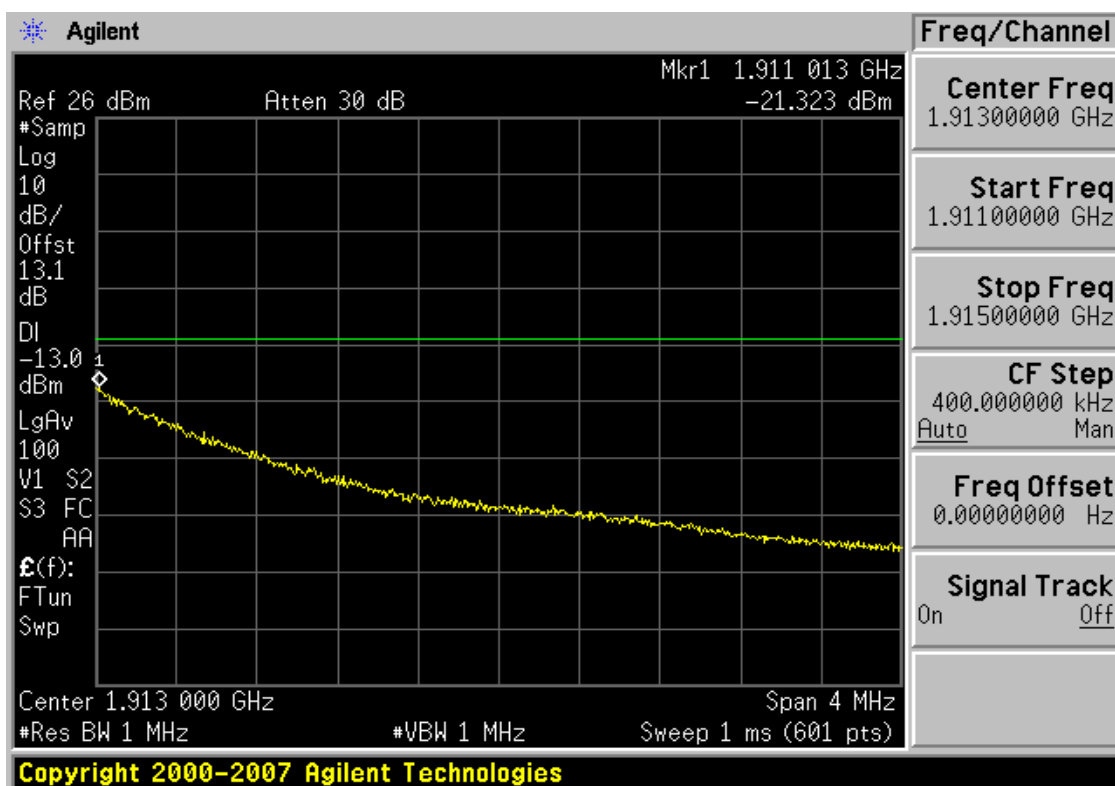
Plot 7-57. 4MHz Span Plot (PCS CDMA Mode – Ch. 1175)
