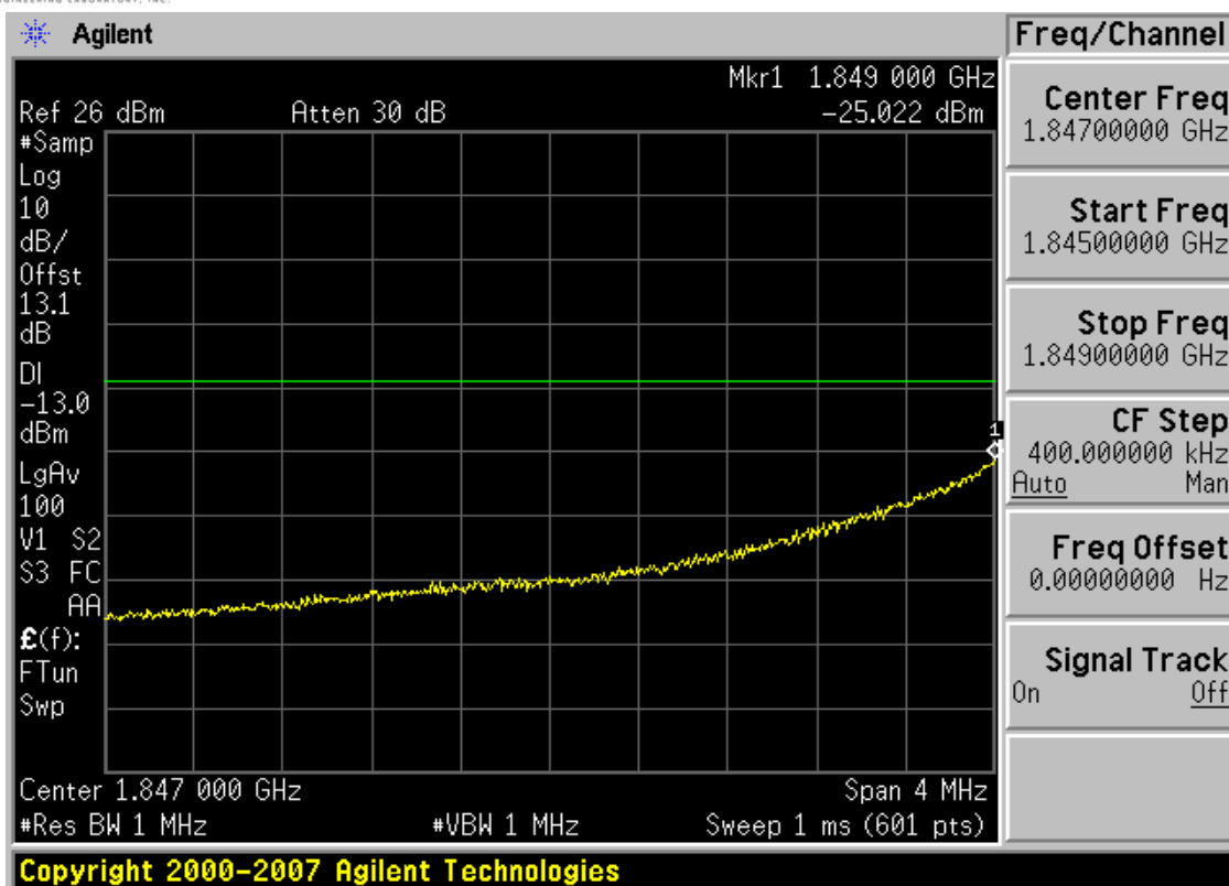
Plot 7-49. 4MHz Span Plot (PCS CDMA Mode – Ch. 25)
