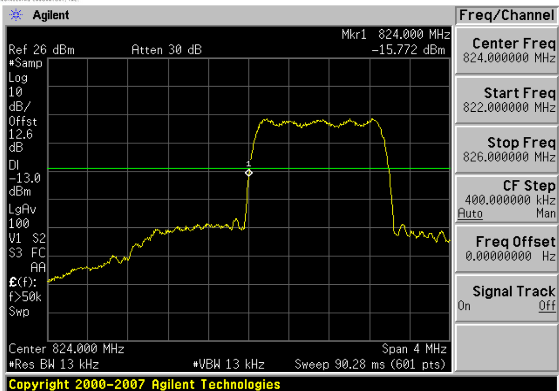
Plot 7-37. Band Edge Plot (Cellular CDMA Mode – Ch. 1013)
