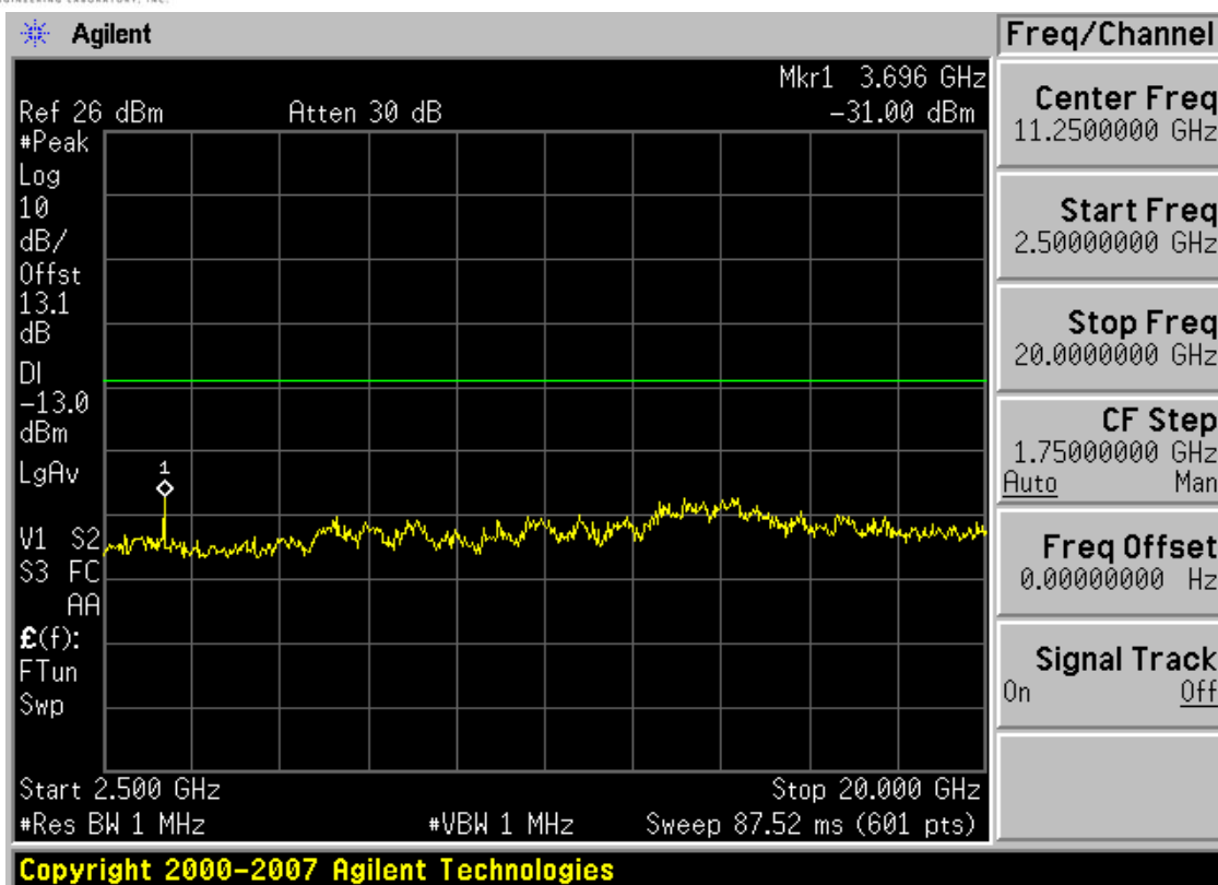
Plot 7-47. Conducted Spurious Plot (PCS CDMA Mode – Ch. 25)
