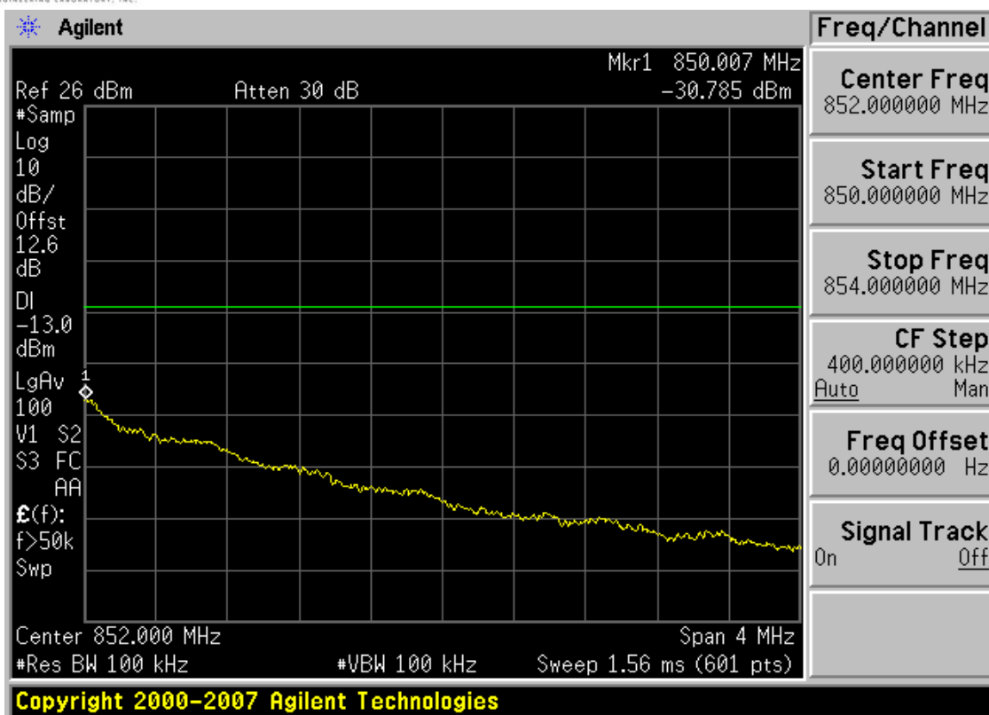
Plot 7-45. 4MHz Span Plot (Cellular CDMA Mode - Ch. 777)
