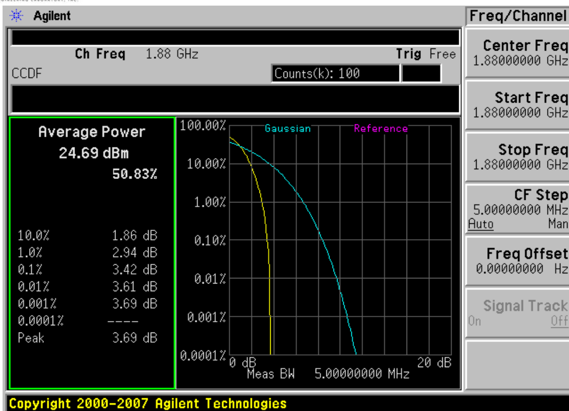
Plot 7-53. Peak-Average Ratio Plot (PCS CDMA Mode - Ch. 600)
