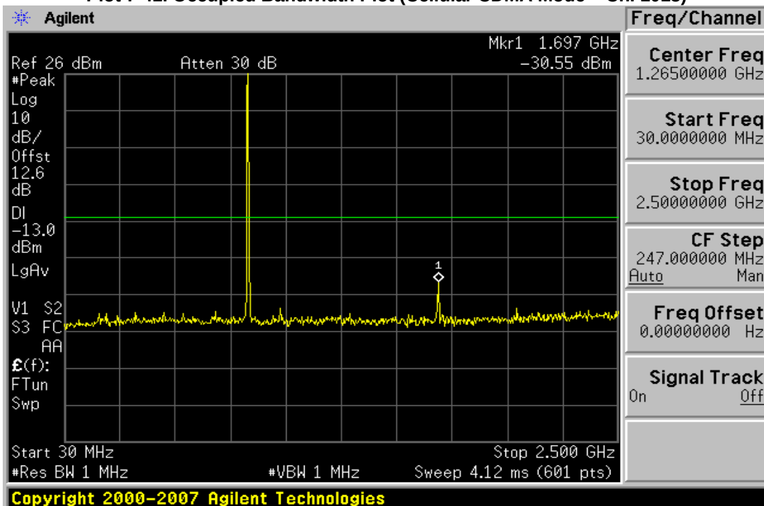
Plot 7-42. Conducted Spurious Plot (Cellular CDMA Mode - Ch. 777)
