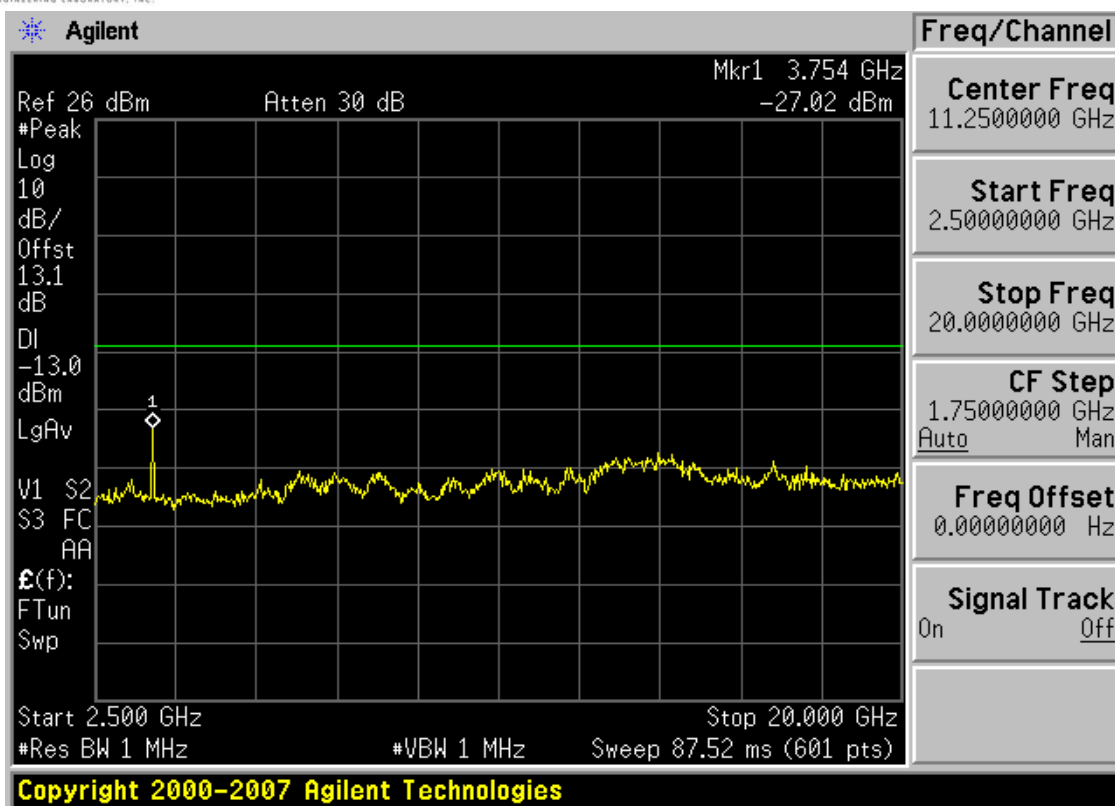
Plot 7-51. Conducted Spurious Plot (PCS CDMA Mode – Ch. 600)
