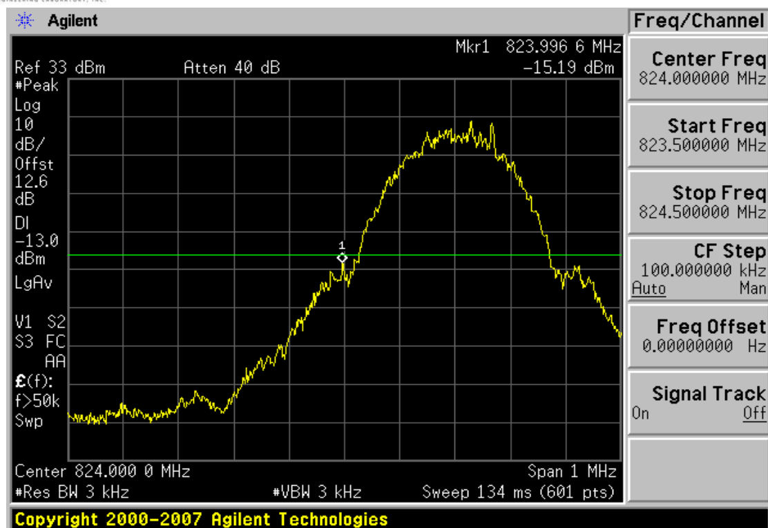
Plot 7-3. Band Edge Plot (Cellular GSM Mode – Ch. 128)
