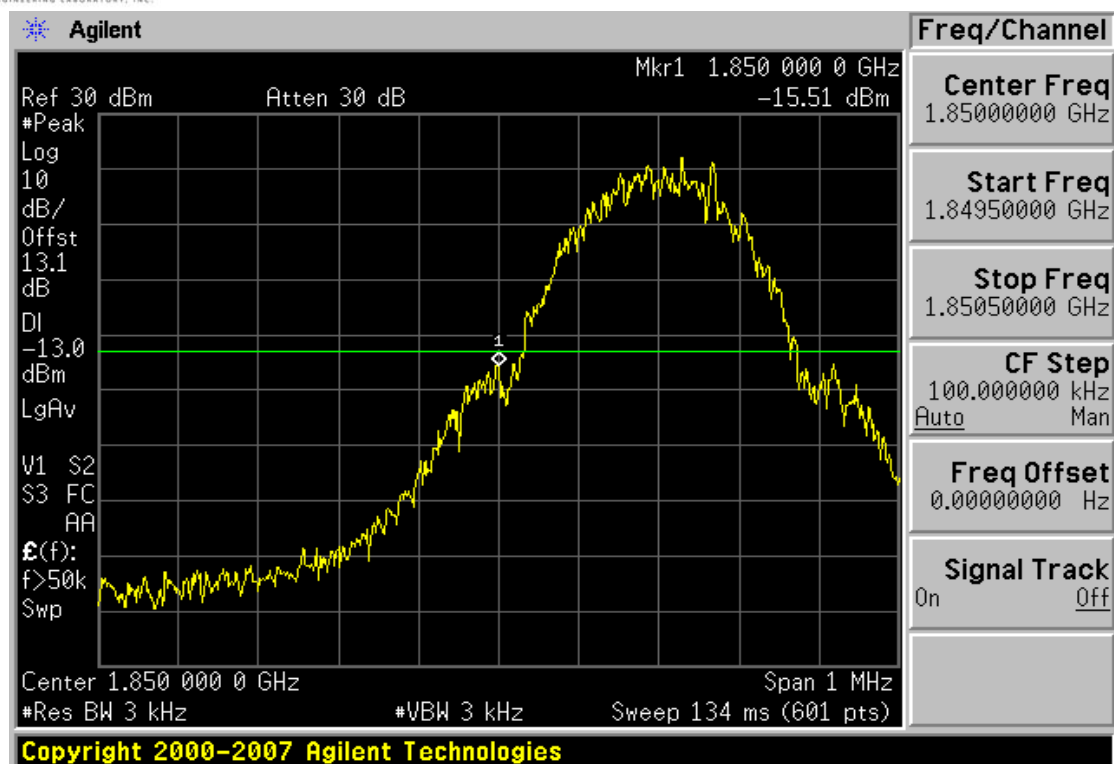
Plot 7-13. Band Edge Plot (PCS GSM Mode – Ch. 512)
