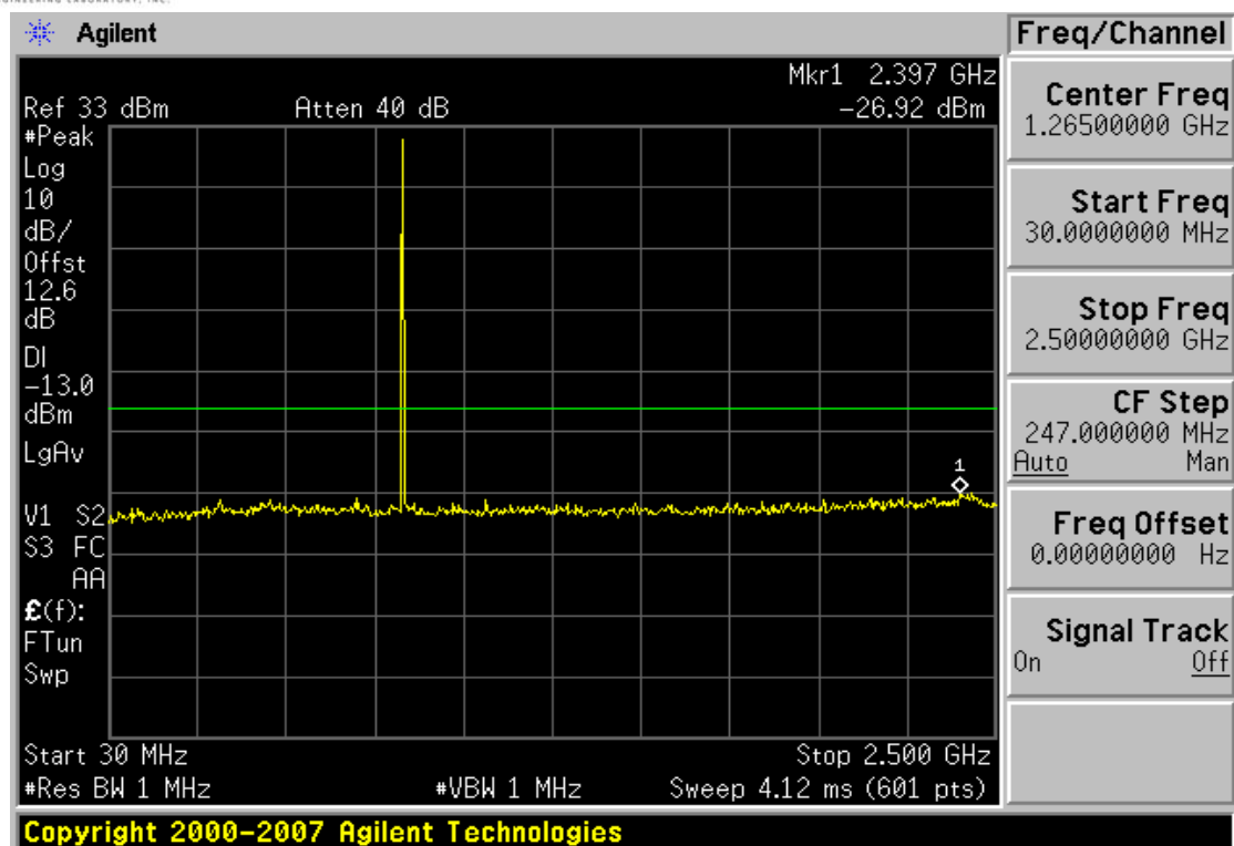
Plot 7-7. Conducted Spurious Plot (Cellular GSM Mode – Ch. 251)
