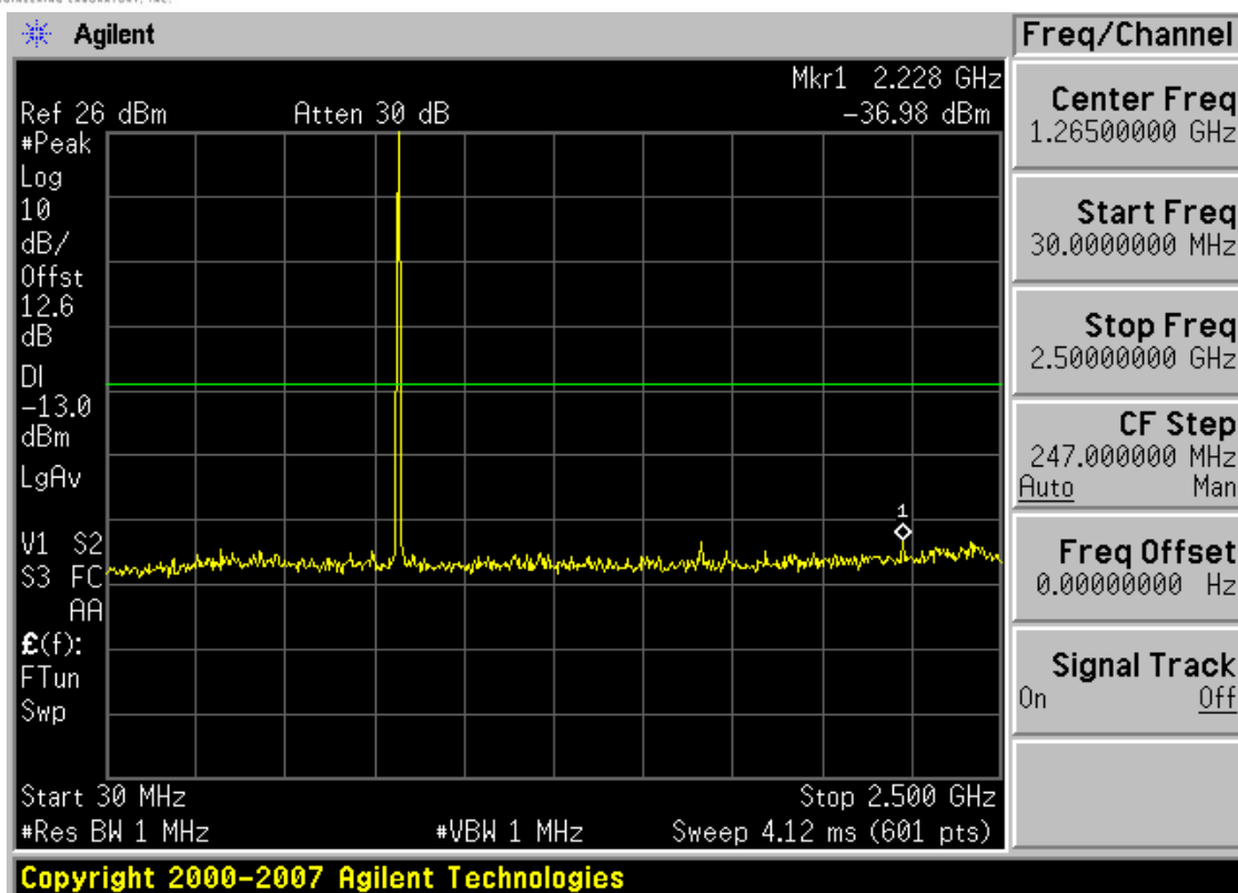
Plot 7-39. Conducted Spurious Plot (Cellular CDMA Mode - Ch. 384)
