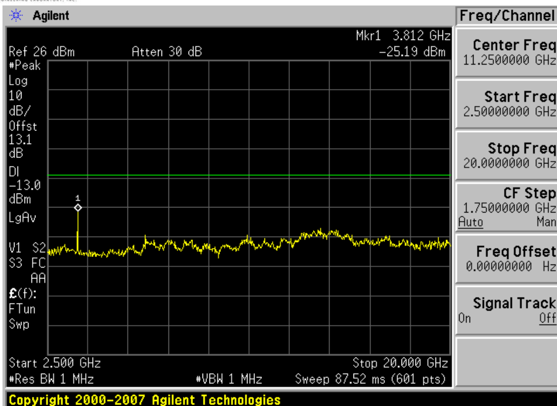
Plot 7-55. Conducted Spurious Plot (PCS CDMA Mode – Ch. 1175)
