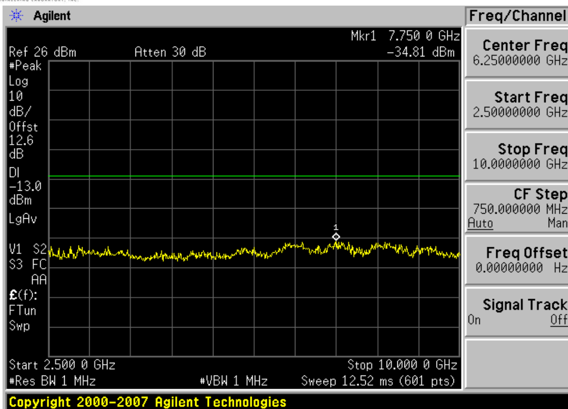
Plot 7-43. Conducted Spurious Plot (Cellular CDMA Mode – Ch. 777)
