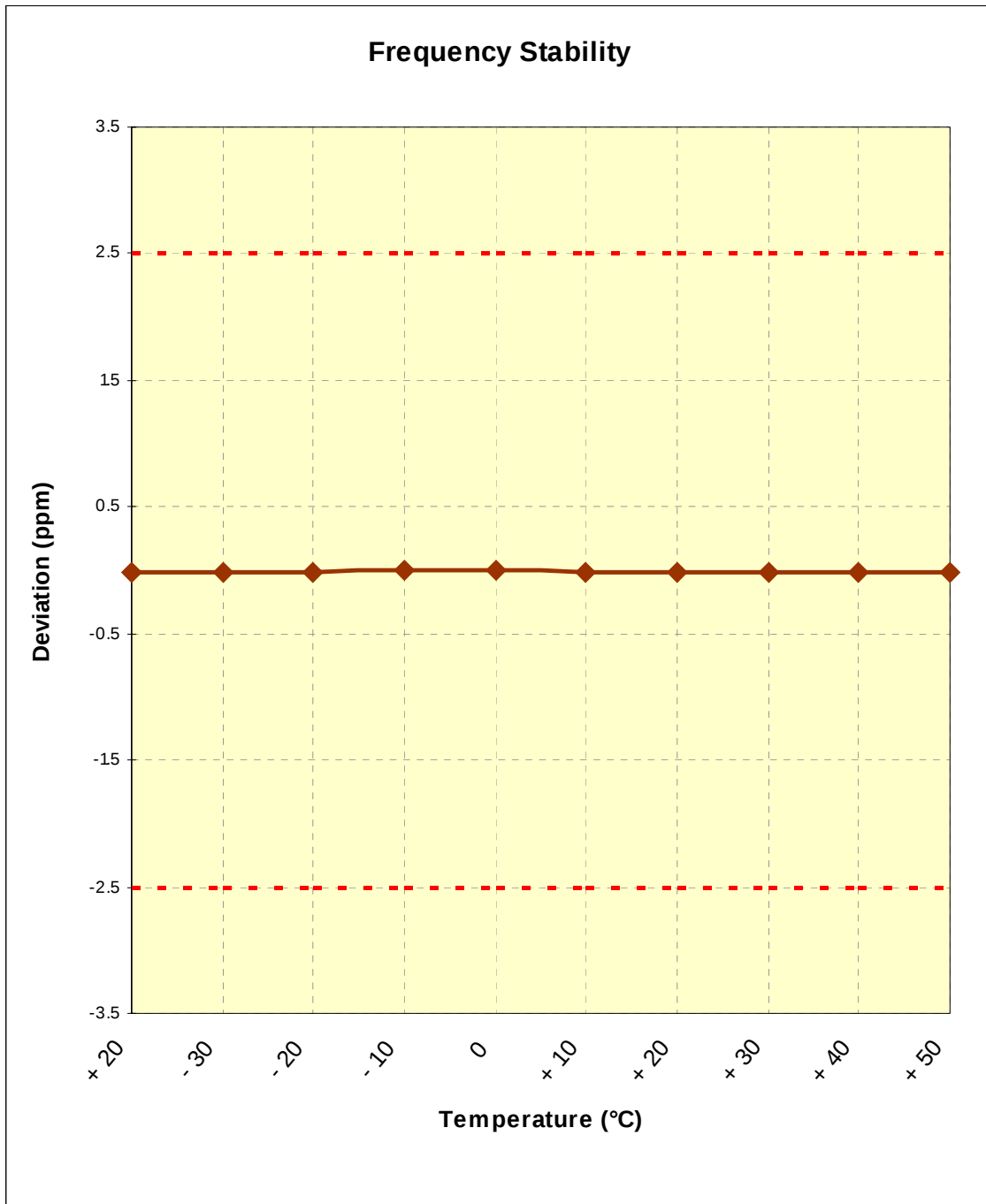
Figure 6-5. Frequency Stability Graph (PCS CDMA Mode – Ch. 600)
