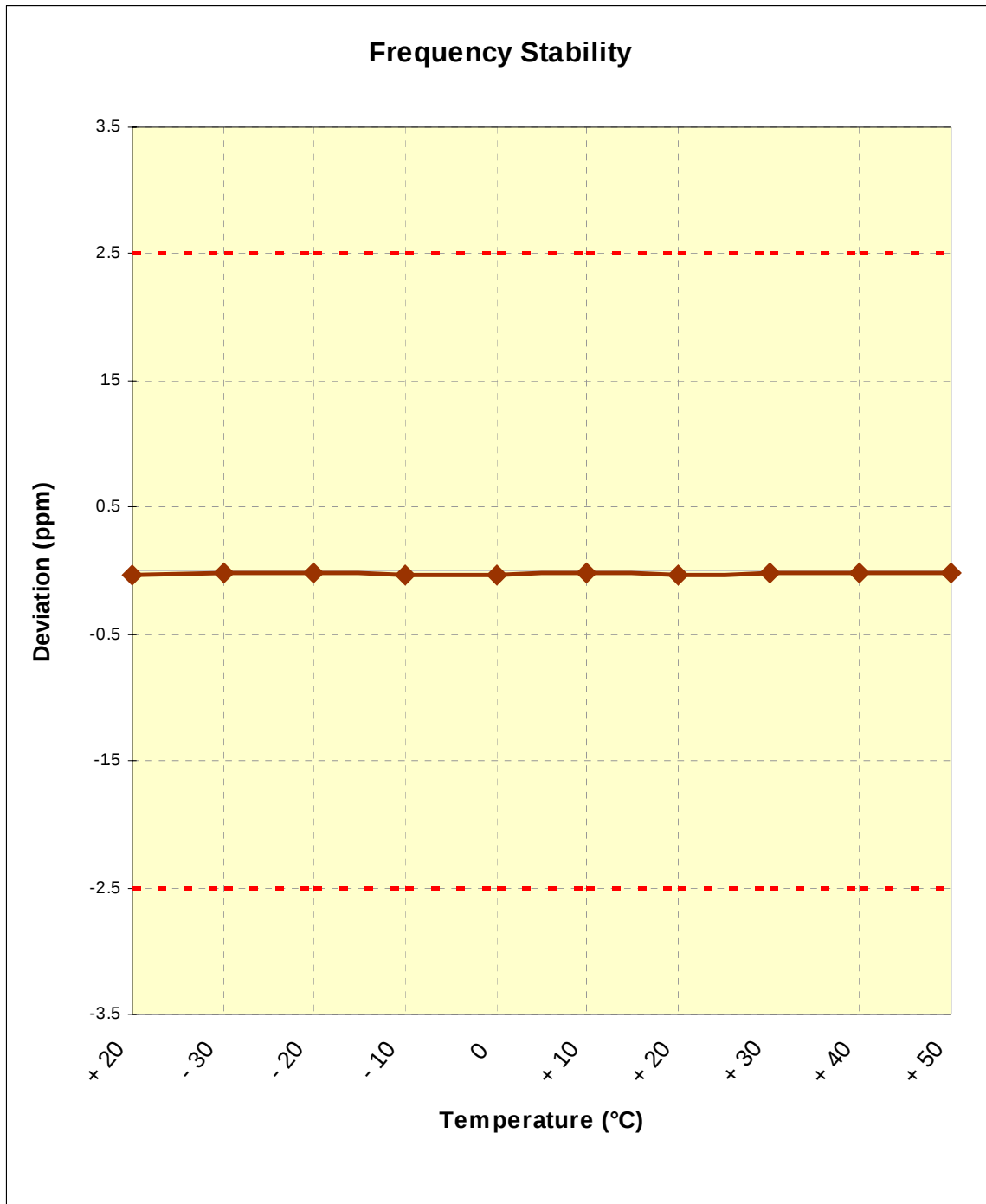
Figure 6-2. Frequency Stability Graph (Cellular CDMA Mode – Ch. 384)
