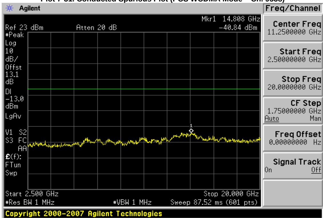
Plot 7-32. Conducted Spurious Plot (PCS WCDMA Mode – Ch. 9538)
