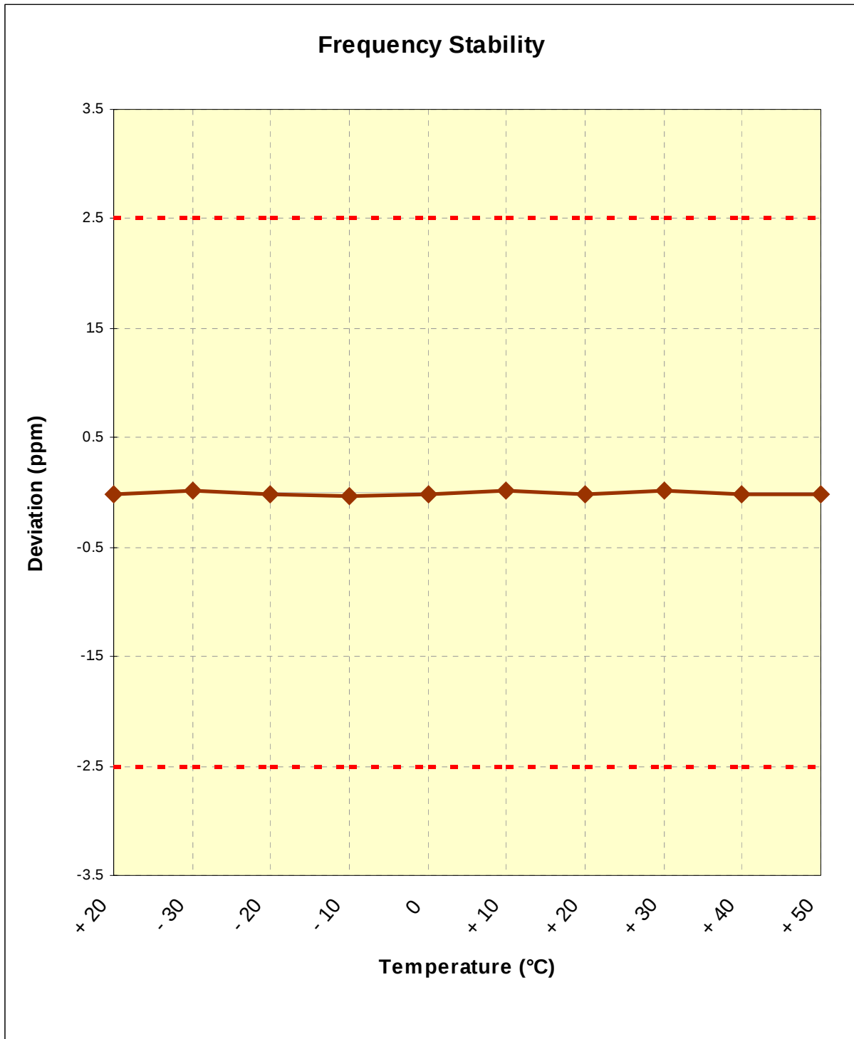
Figure 6-1. Frequency Stability Graph (Cellular GSM Mode – Ch. 190)
