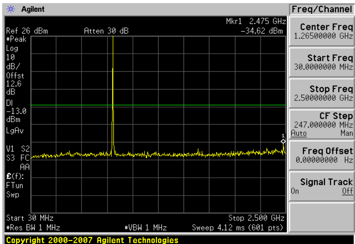
Plot 7-35. Conducted Spurious Plot (Cellular CDMA Mode – Ch. 1013)
