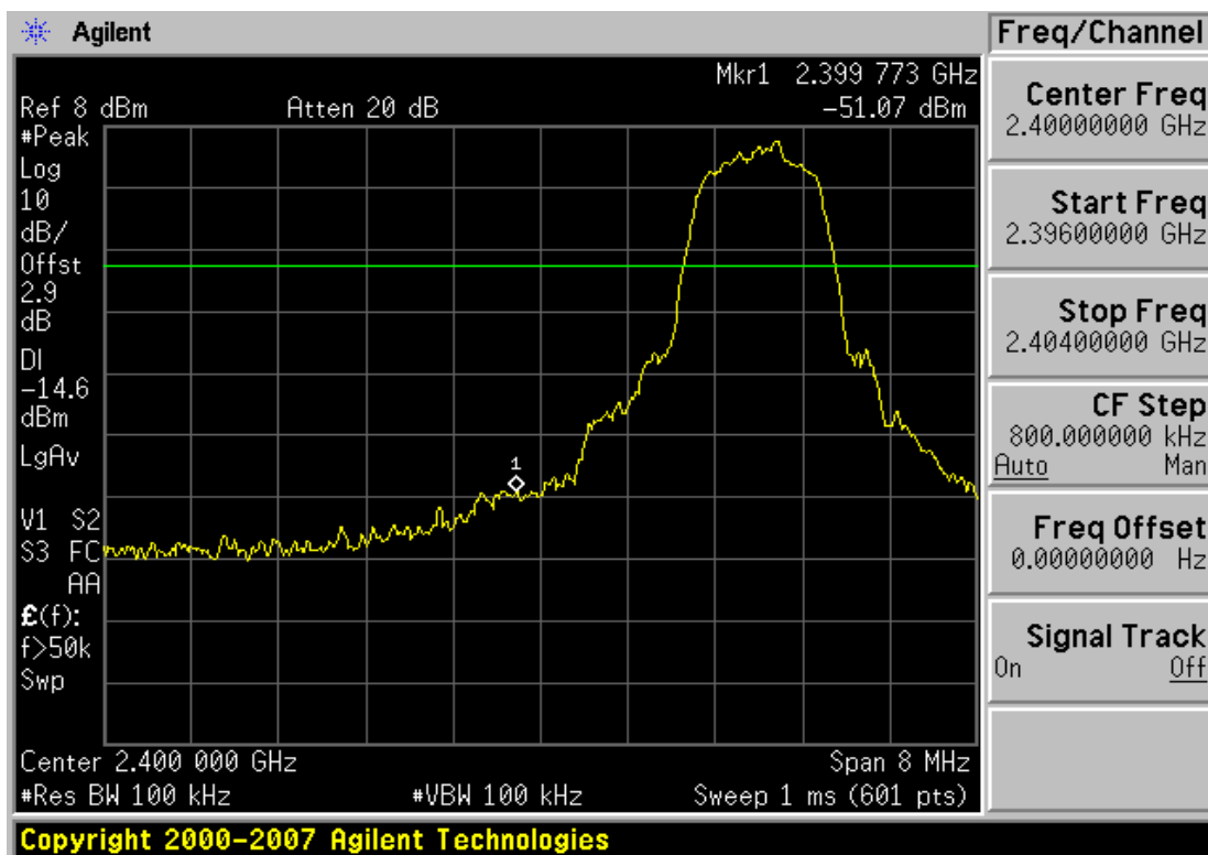
Plot 6-6. Band Edge Plot (Bluetooth (EDR) - Ch. 0)
