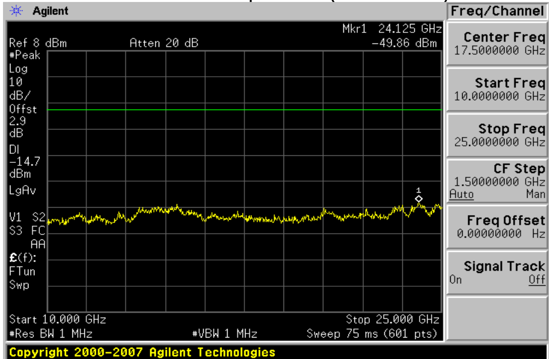
Plot 6-13. Conducted Spurious Plot (Bluetooth – Ch. 0)
