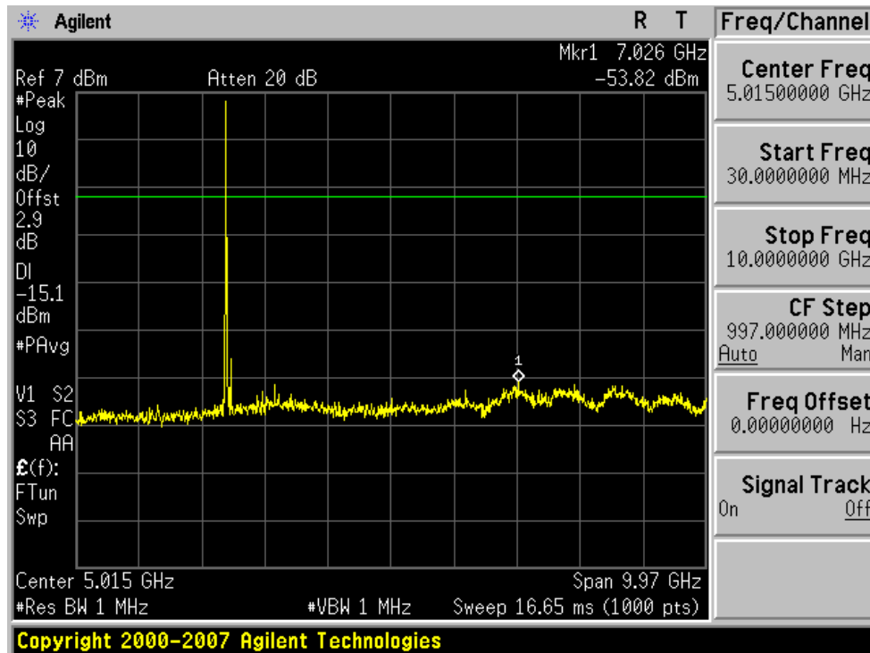
Plot 6-2. Conducted Spurious Plot (Bluetooth – Ch. 0)
