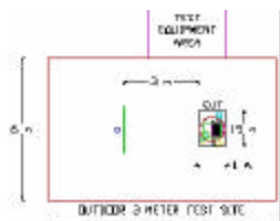
Figure 3-2. Dimensions of Outdoor Test Site
