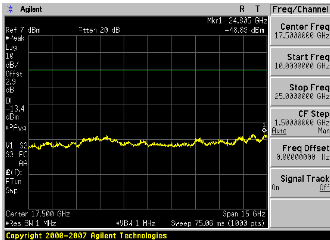
Plot 6-7. Conducted Spurious Plot (Bluetooth – Ch. 78)
