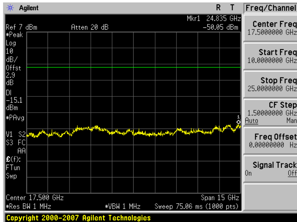
Plot 6-3. Conducted Spurious Plot (Bluetooth – Ch. 0)
