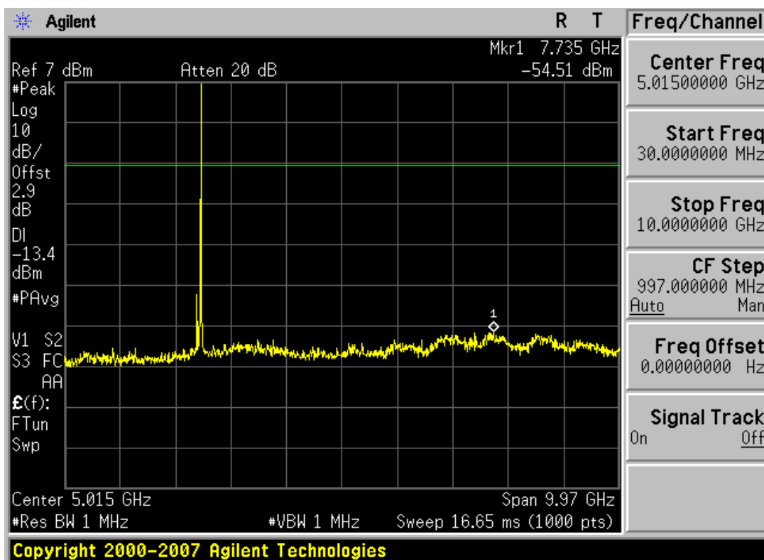
Plot 6-6. Conducted Spurious Plot (Bluetooth – Ch. 78)
