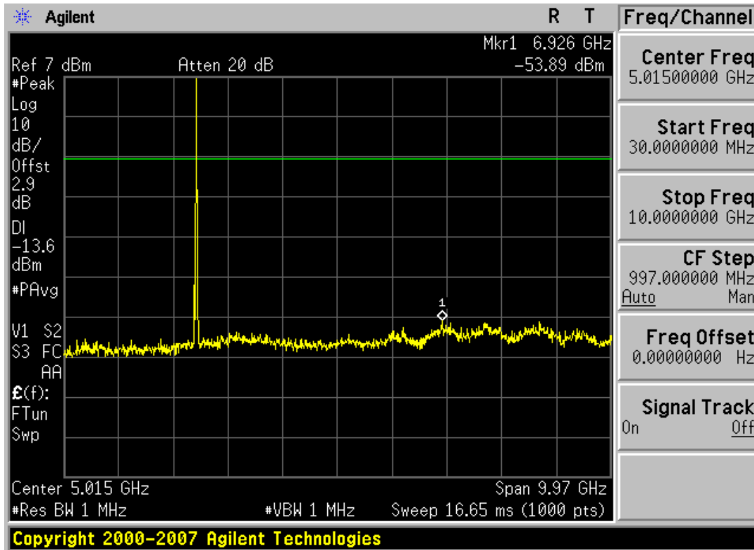
Plot 6-4. Conducted Spurious Plot (Bluetooth – Ch. 39)
