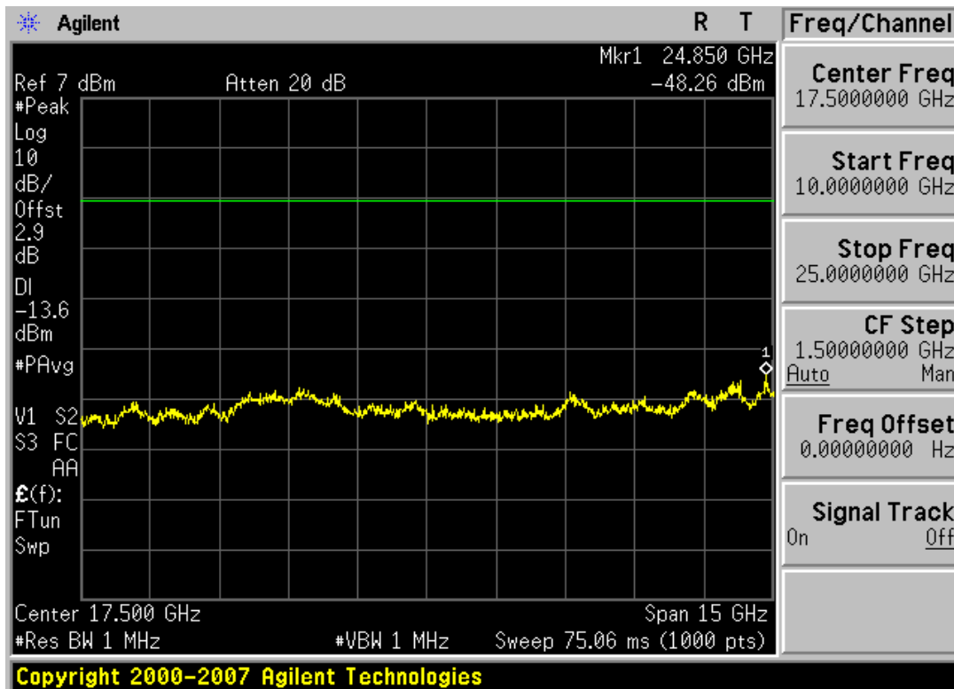
Plot 6-5. Conducted Spurious Plot (Bluetooth – Ch. 39)
