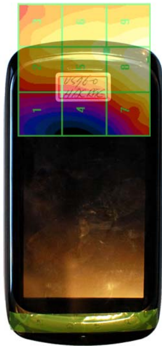
Figure 17-4 E-Field WD Scan overlay
