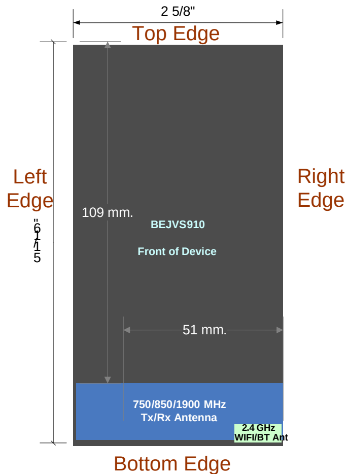
Figure 16-1 Identification of Sides/Edges for SAR Testing (Front View)
