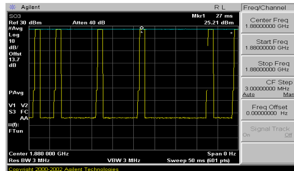
Figure 8-4 Zero-Span Plots
