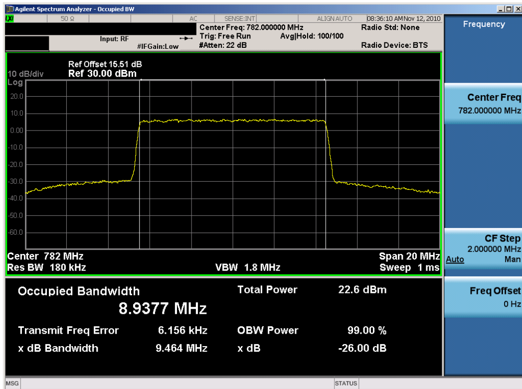
Plot 7-11. Occupied Bandwidth Plot (QPSK – RB Size 50)
