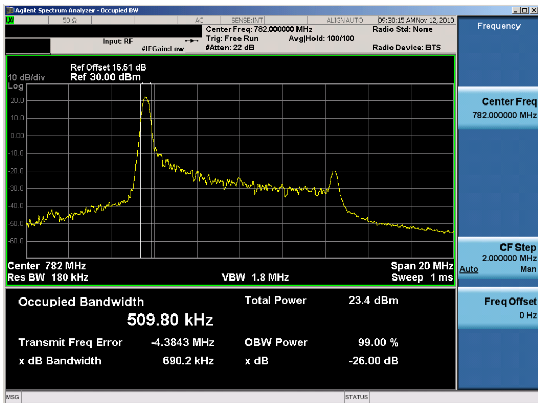
Plot 7-5. Occupied Bandwidth Plot (QPSK – RB Size 1, RB Offset 0)
