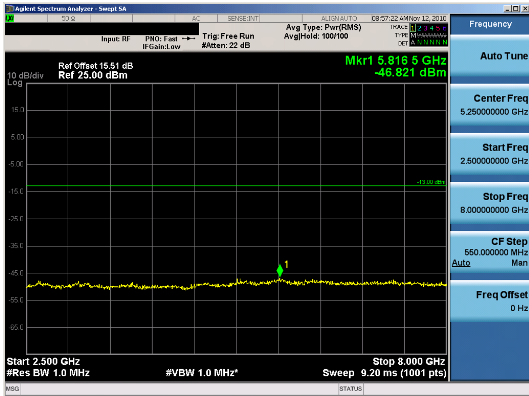
Plot 7-14. Conducted Spurious Plot (QPSK – RB Size 50)
