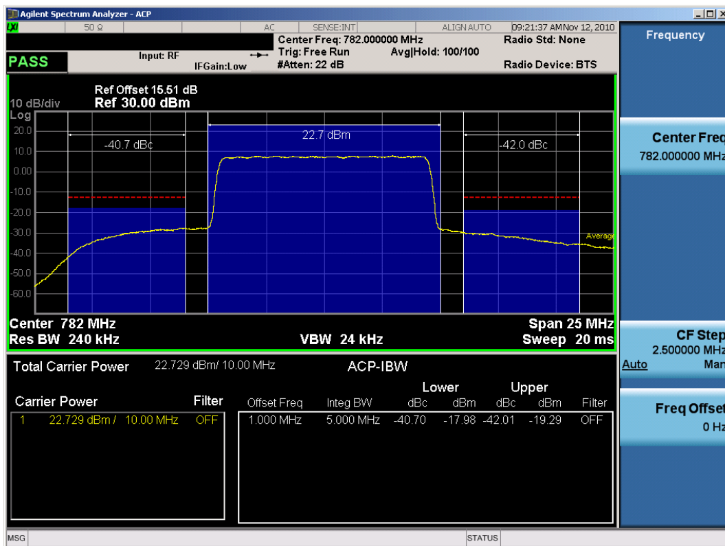
Plot 7-1. Lower/Upper Band Edge Plot (QPSK – RB Size 50)
