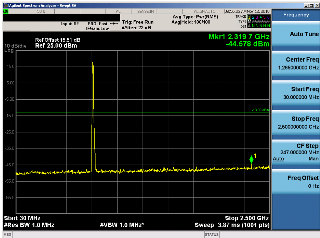
Plot 7-13. Conducted Spurious Plot (QPSK – RB Size 50)
