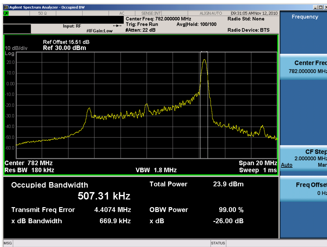
Plot 7-7. Occupied Bandwidth Plot (QPSK – RB Size 1, RB Offset 49)
