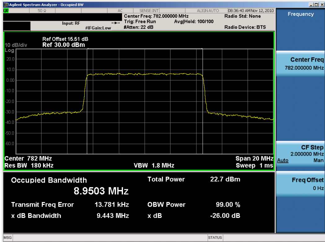
Plot 7-12. Occupied Bandwidth Plot (16-QAM – RB Size 50)
