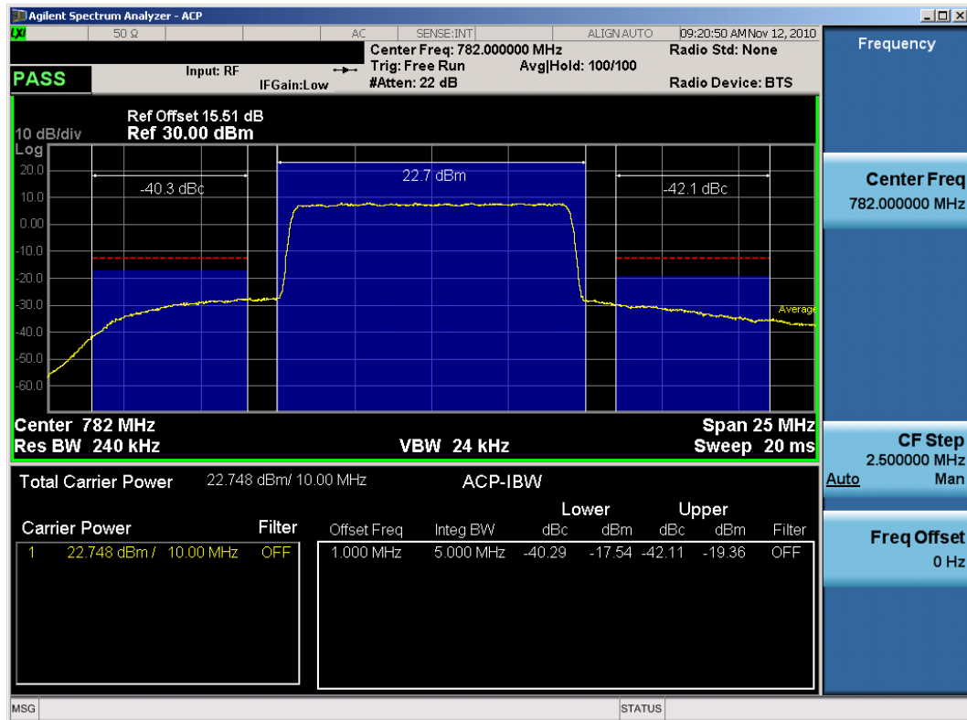
Plot 7-2. Lower/Upper Band Edge Plot (16-QAM – RB Size 50)
