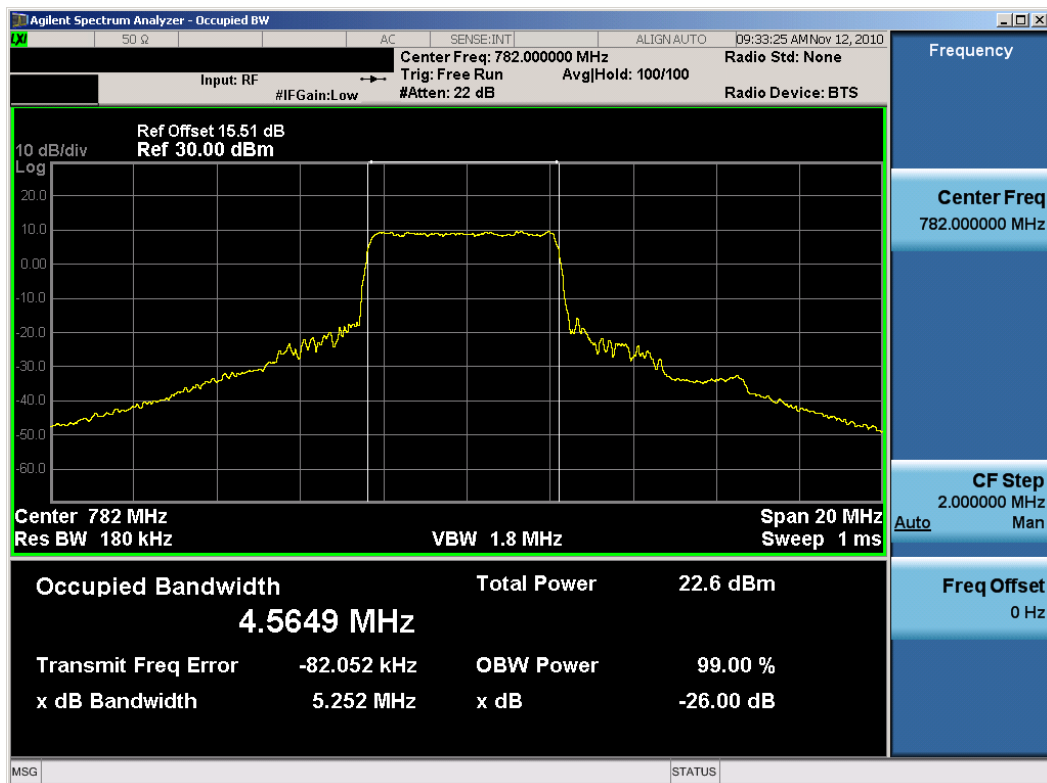
Plot 7-9. Occupied Bandwidth Plot (QPSK – RB Size 25, RB Offset 12)
