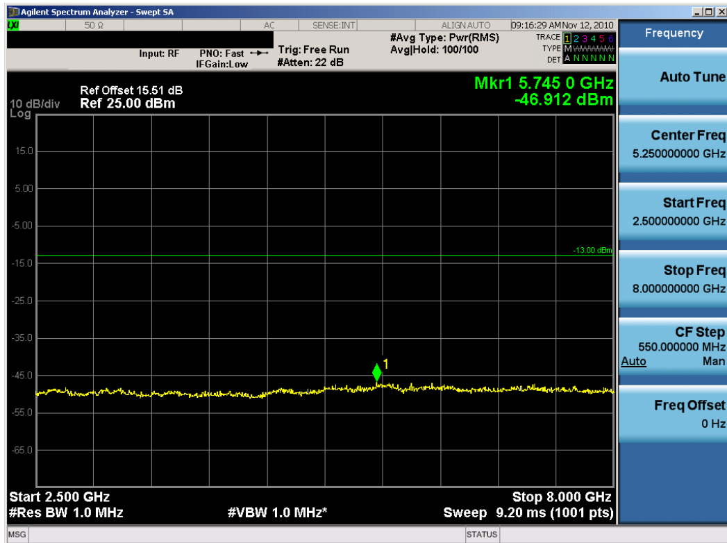
Plot 7-16. Conducted Spurious Plot (16-QAM – RB Size 50)
