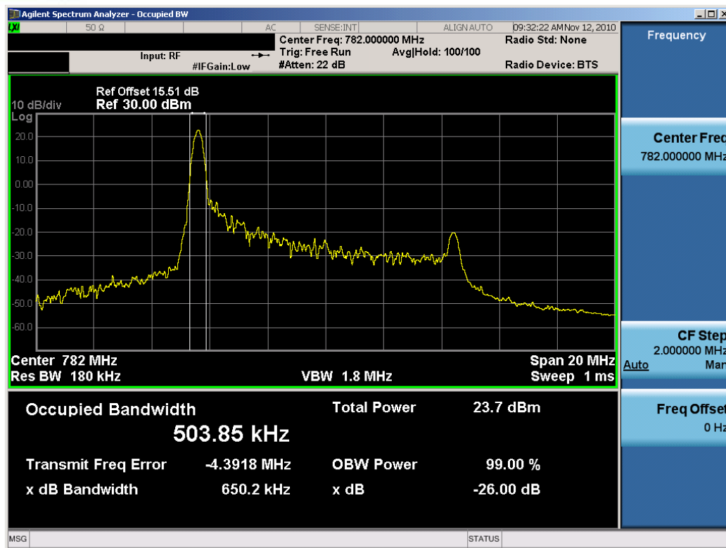
Plot 7-6. Occupied Bandwidth Plot (16-QAM – RB Size 1, RB Offset 0)
