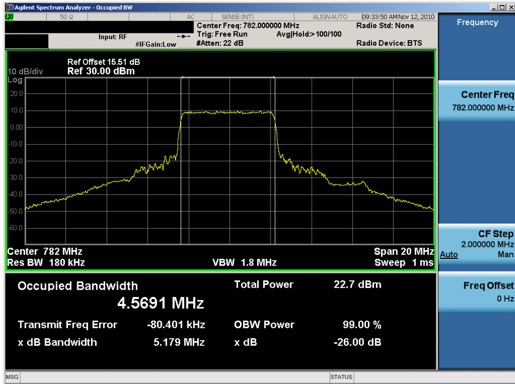
Plot 7-10. Occupied Bandwidth Plot (16-QAM – RB Size 25, RB Offset 12)
