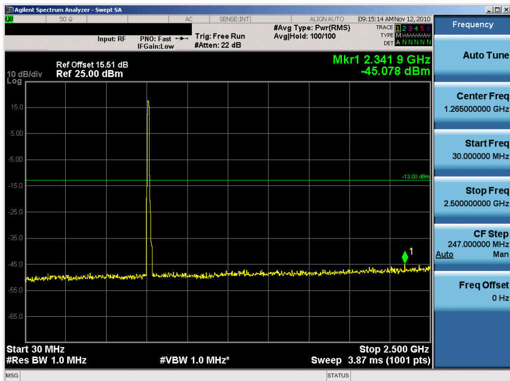
Plot 7-15. Conducted Spurious Plot (16-QAM – RB Size 50)
