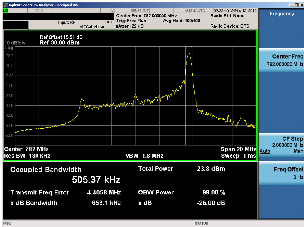
Plot 7-8. Occupied Bandwidth Plot (16-QAM – RB Size 1, RB Offset 49)
