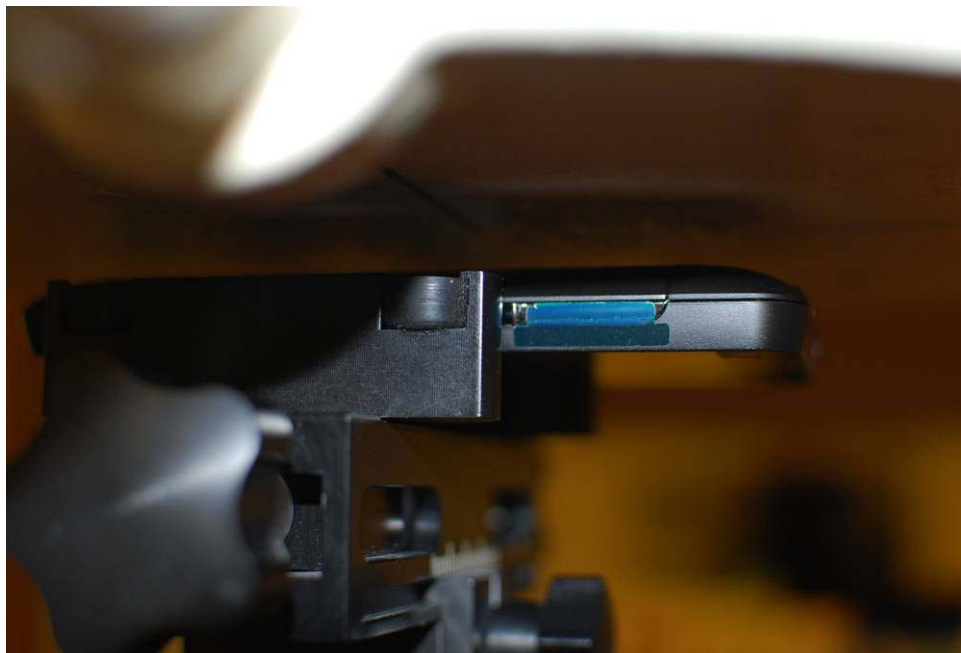
Figure 23-6 SAR Test Setup Photo 6 – Back at 1.0 cm
