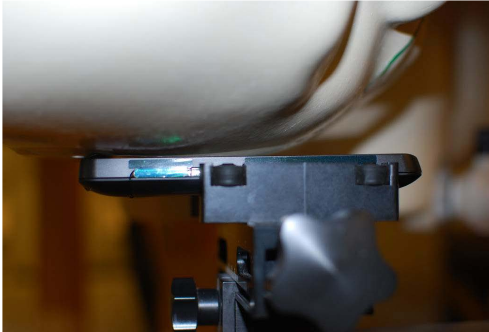
Figure 22-1 SAR Test Setup Photo 1
