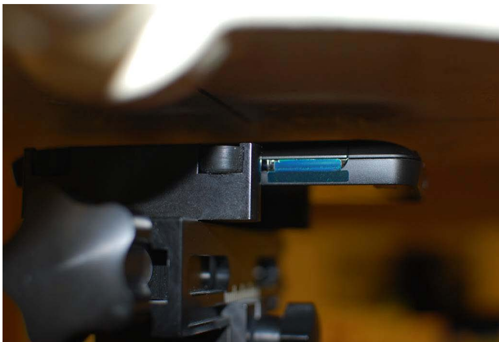
Figure 22-5 SAR Test Setup Photo 6: Back Side
