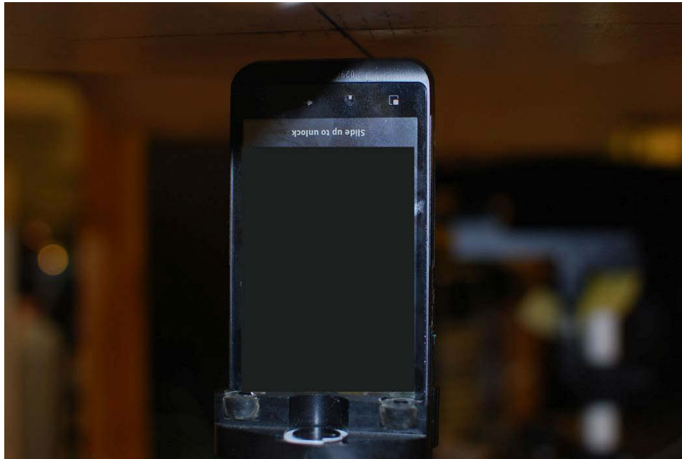
Figure 22-9 SAR Test Setup Photo 10: Bottom Edge
